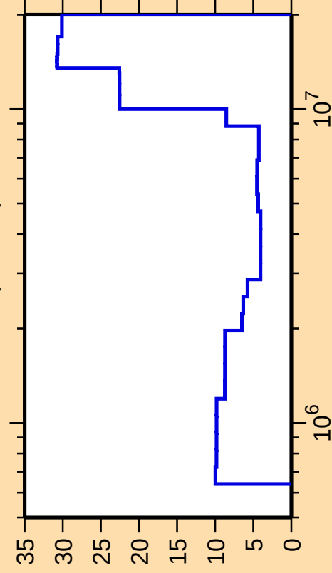
\Delta\sigma/\sigma vs. E for ^{82}\text{Se}(\text{n,inel.})
