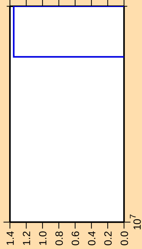
\Delta\sigma/\sigma vs. E for ^{82}\text{Se}(n,\text{nt})
