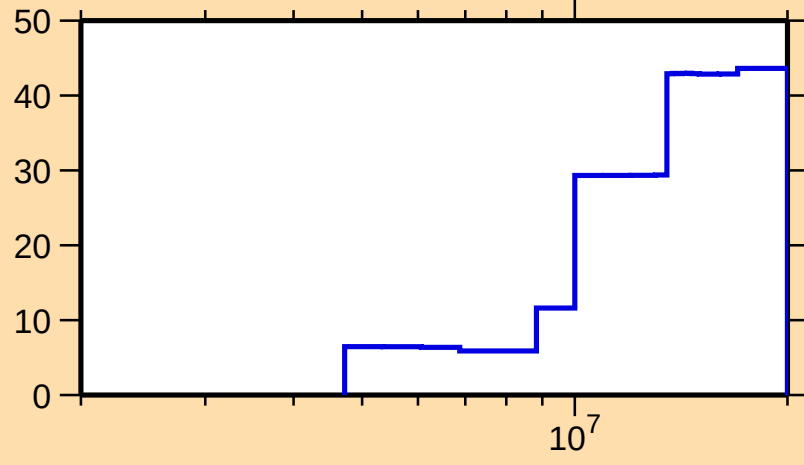
\Delta\sigma/\sigma vs. E for ^{82}\text{Se}(n,n\text{cont.})
