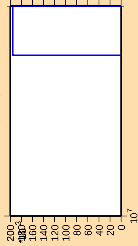
\Delta\sigma/\sigma vs. E for ^{82}\text{Se}(n,\text{nd})
