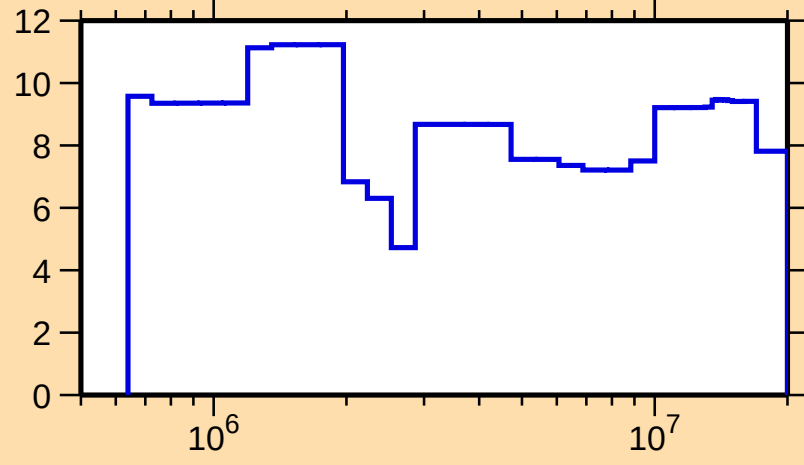
\Delta\sigma/\sigma vs. E for ^{82}\text{Se}(\text{n,el.})
