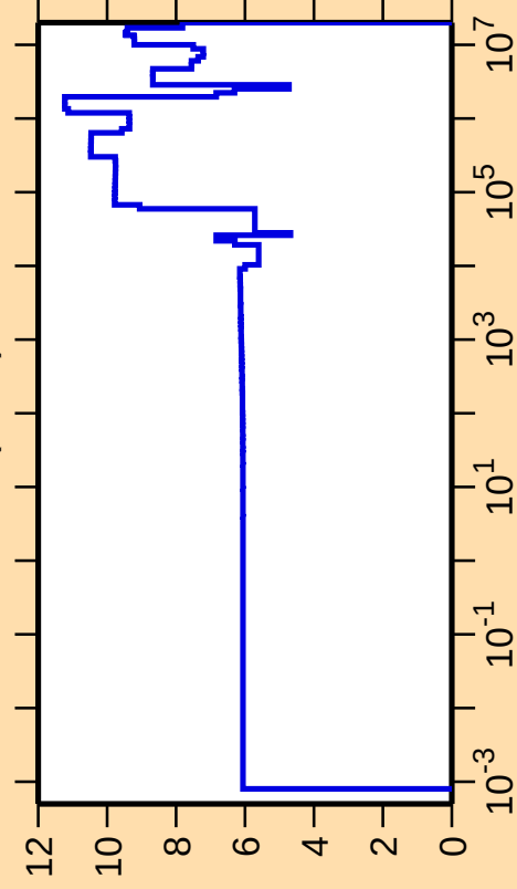
\Delta\sigma/\sigma vs. E for ^{82}\text{Se}(n,\text{el.})
