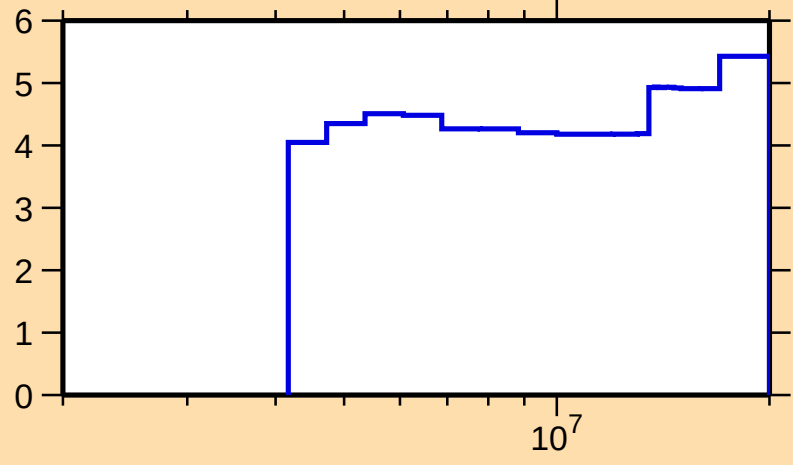
\Delta\sigma/\sigma vs. E for ^{82}\text{Se}(n,n\text{onel.})
