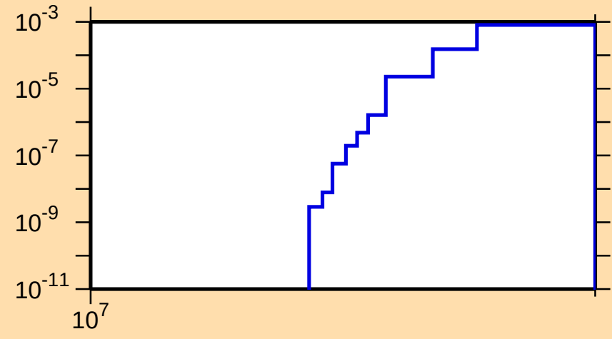
\sigma vs. E for ^{82}\text{Se}(n,np)
