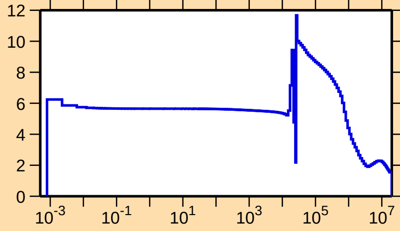
\sigma vs. E for ^{82}\text{Se}(n,\text{el.})
