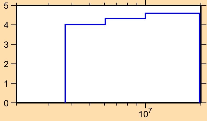
\Delta\sigma/\sigma vs. E for ^{82}\text{Se}(n,n\text{nonel.})
