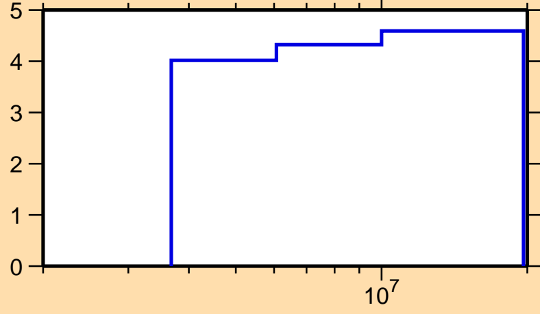
\Delta\sigma/\sigma vs. E for ^{82}\text{Se}(n,\text{nonel.})
