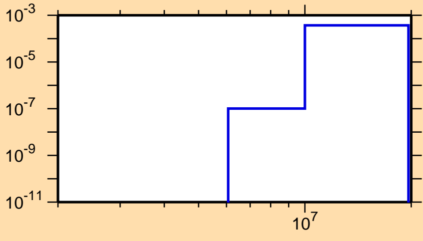
\sigma vs. E for ^{82}\text{Se}(n,\alpha)
