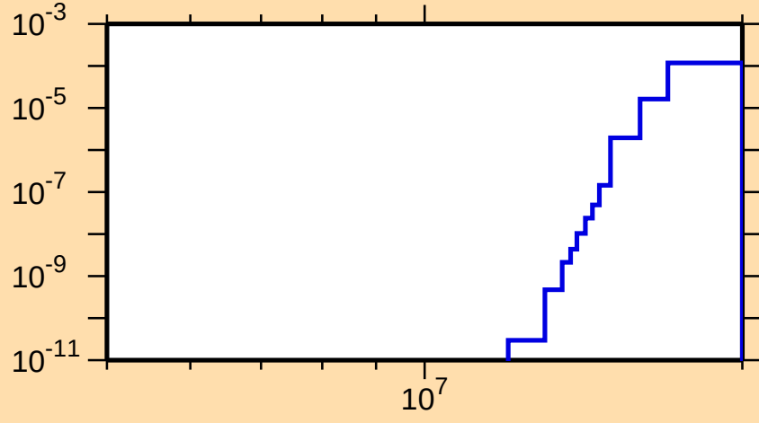
\sigma vs. E for ^{83}\text{Se}(n,n\alpha)
