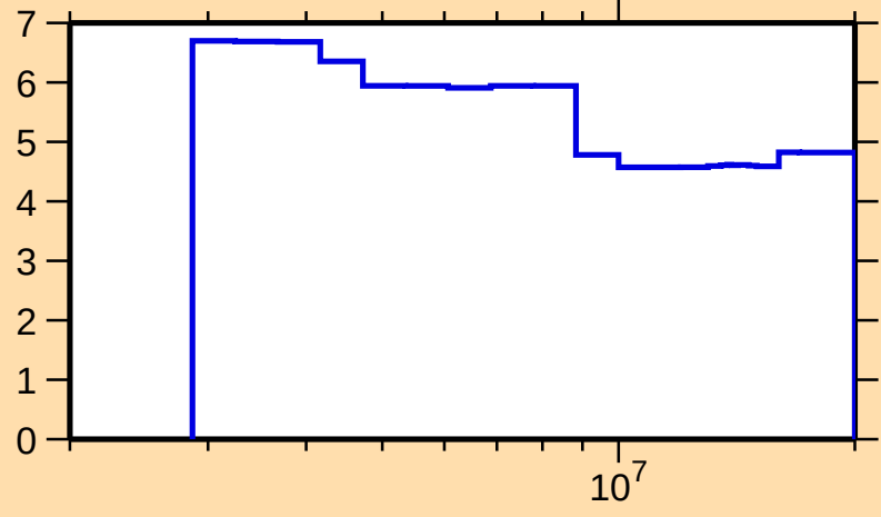
\Delta\sigma/\sigma vs. E for ^{83}\text{Se}(n,n\text{onel.})
