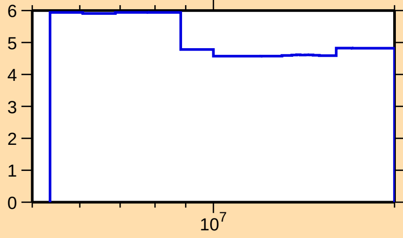
\Delta\sigma/\sigma vs. E for ^{83}\text{Se}(n,\text{nonel.})
