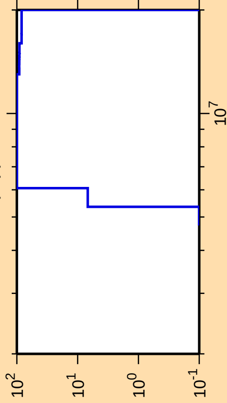
\Delta\sigma/\sigma vs. E for ^{83}\text{Se}(n,p)
