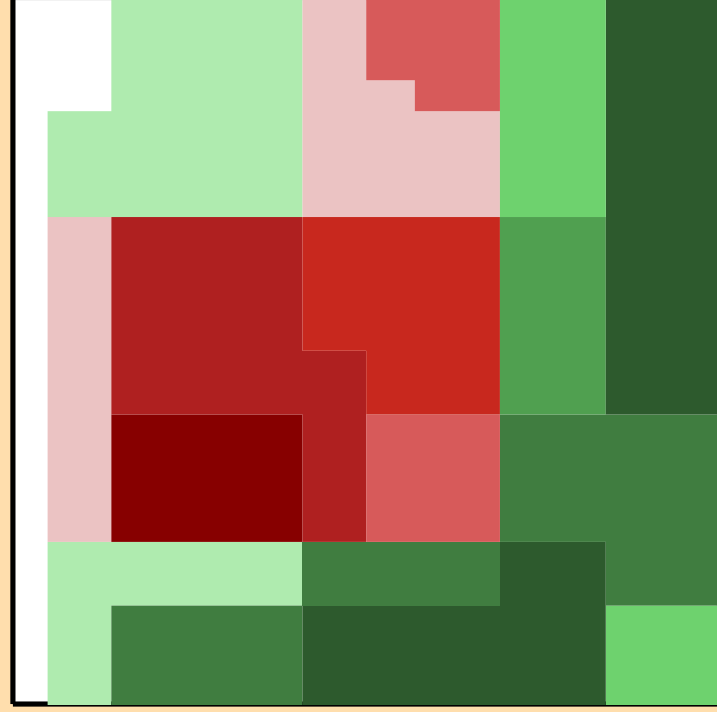
\Delta\sigma/\sigma vs. E for ^{83}\text{Se}(n,2n)
