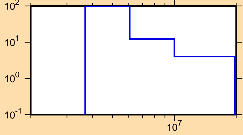
\Delta\sigma/\sigma vs. E for ^{83}\text{Se}(n,2n)
