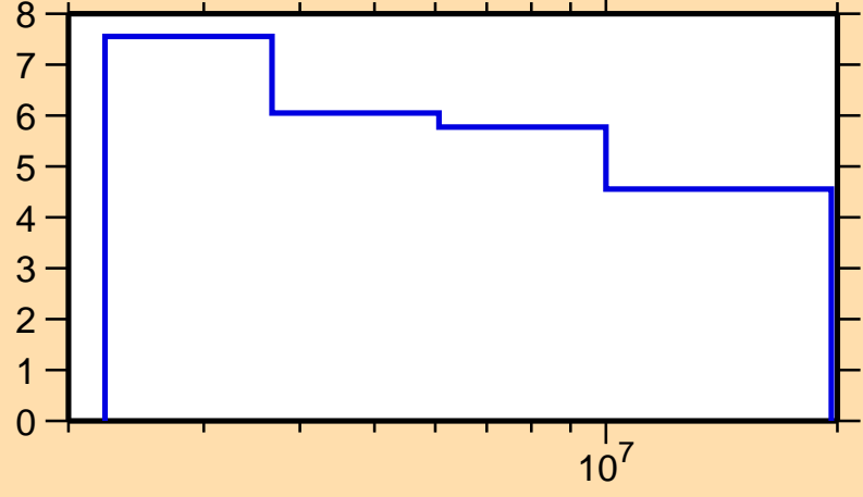
\Delta\sigma/\sigma vs. E for ^{83}\text{Se}(n,n\text{nonel.})
