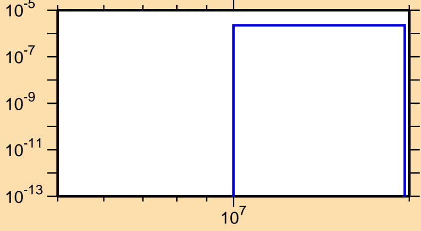
\sigma vs. E for ^{83}\text{Se}(n,\alpha)
