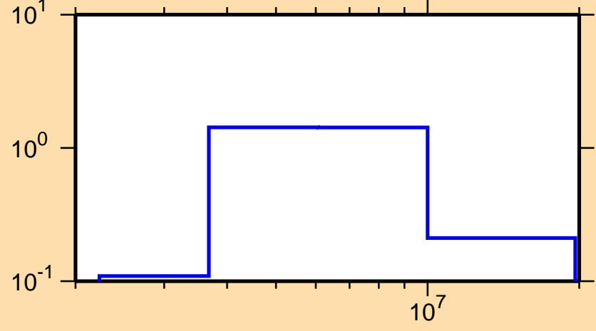
\sigma vs. E for ^{83}\text{Se}(n,n\text{cont.})
