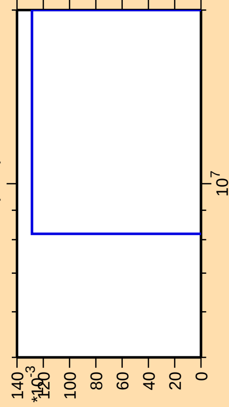
\Delta\sigma/\sigma vs. E for ^{83}\text{Se}(n,nt)
