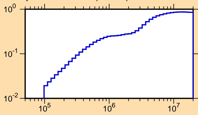
\mu vs. E for ^{84}\text{Se}(\text{mt251})
