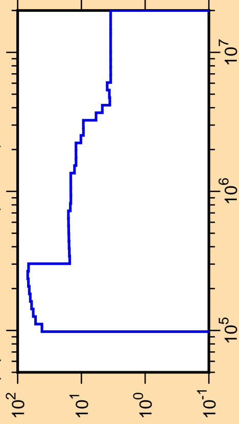
\Delta\mu/\mu vs. E for ^{84}\text{Se}(\text{mt251})
