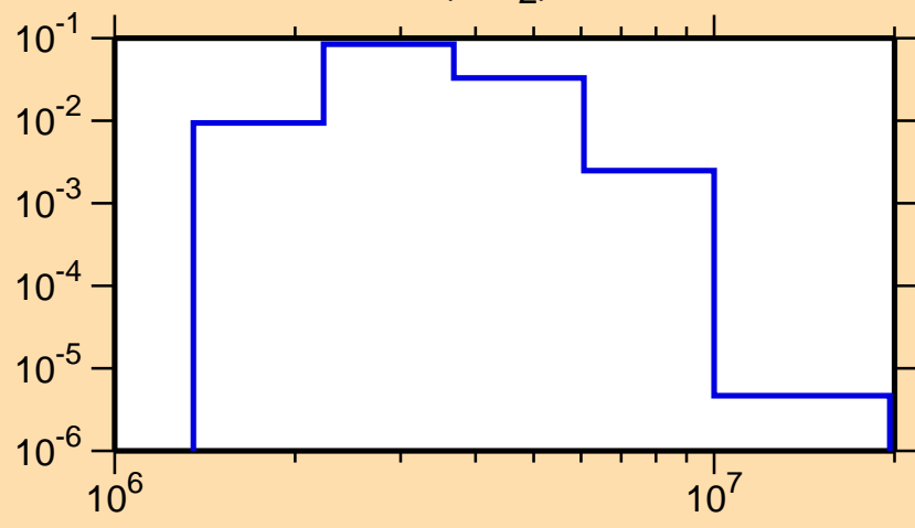
\sigma vs. E for ^{84}\text{Se}(n,n_2)
