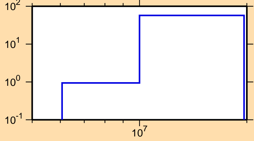
\Delta\sigma/\sigma vs. E for ^{84}\text{Se}(n,p)
