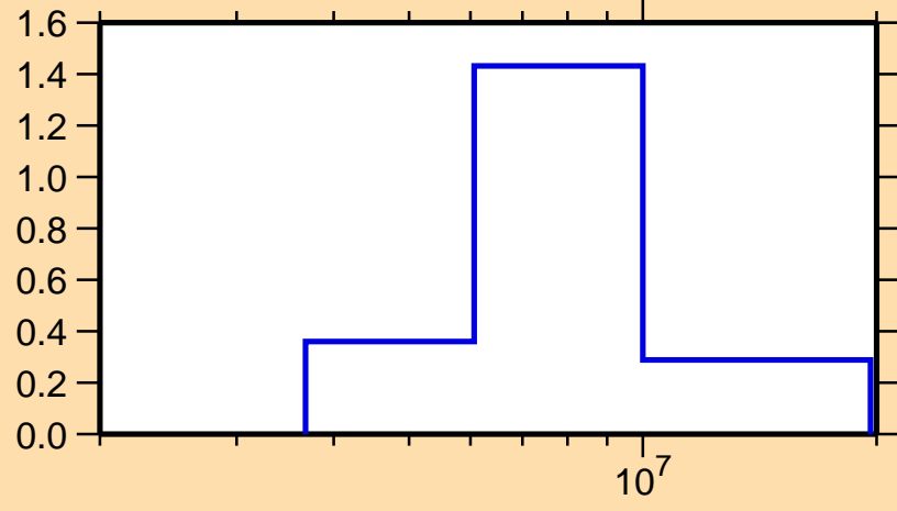
\sigma vs. E for ^{84}\text{Se}(n,n\text{cont.})
