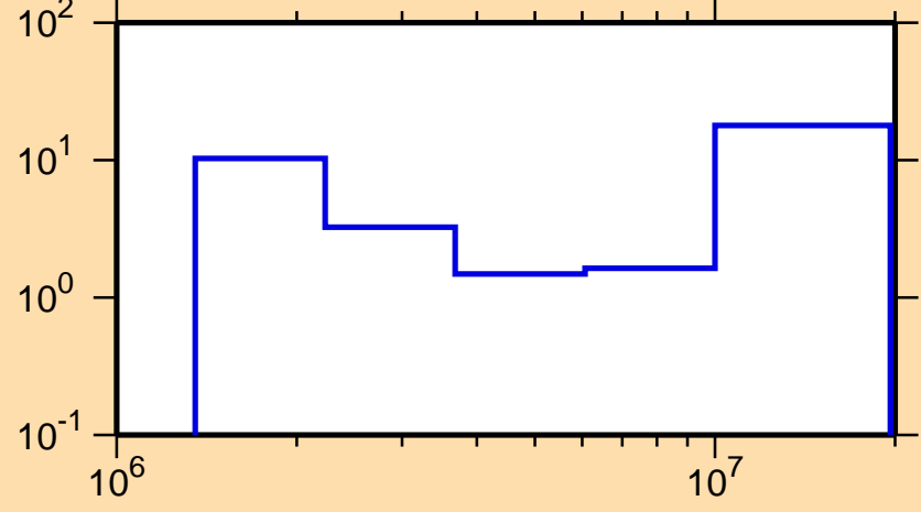
\Delta\sigma/\sigma vs. E for ^{84}\text{Se}(n,\text{inel.})
