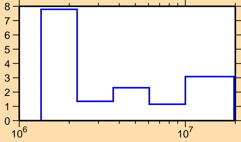
\Delta\sigma/\sigma vs. E for ^{84}\text{Se}(n,\text{tot.})
