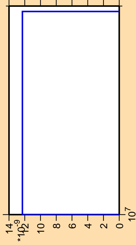
\Delta\sigma/\sigma vs. E for ^{84}\text{Se}(n,\text{nd})
