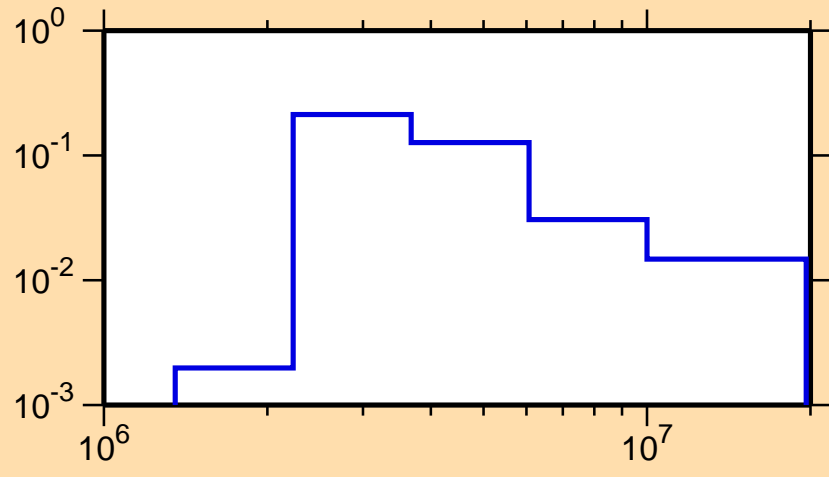
\sigma vs. E for ^{84}\text{Se}(n,n_4)
