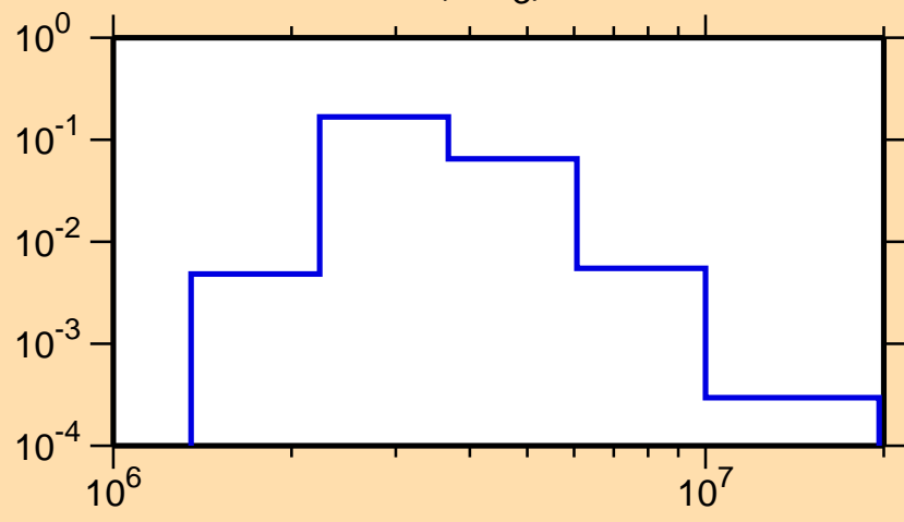
\sigma vs. E for ^{84}\text{Se}(n,n_3)
