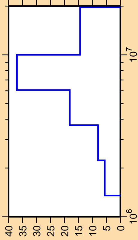
\Delta\sigma/\sigma vs. E for ^{84}\text{Se}(n,n_3)
