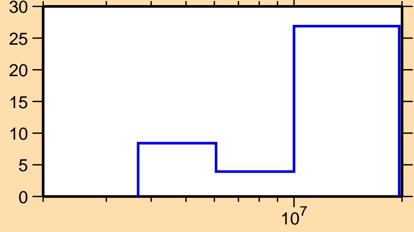
\Delta\sigma/\sigma vs. E for ^{84}\text{Se}(n,ncont.)
