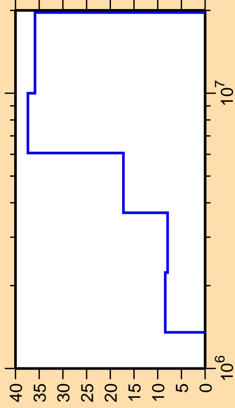
\Delta\sigma/\sigma vs. E for ^{84}\text{Se}(n,n_2)
