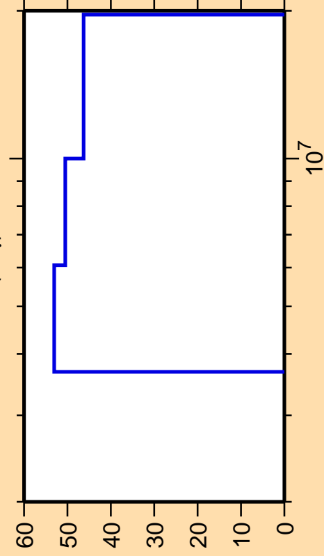
\Delta\sigma/\sigma vs. E for ^{84}\text{Se}(n,\gamma)
