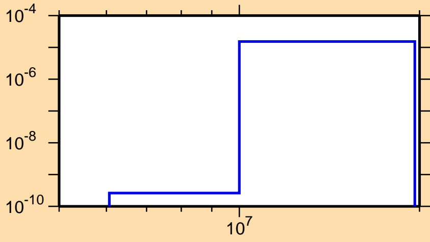
\sigma vs. E for ^{84}\text{Se}(n,\alpha)
