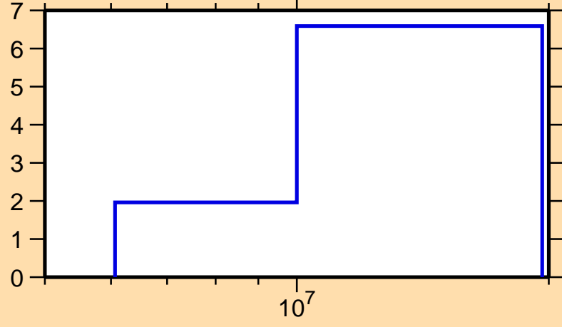
\Delta\sigma/\sigma vs. E for ^{84}\text{Se}(n,el.)
