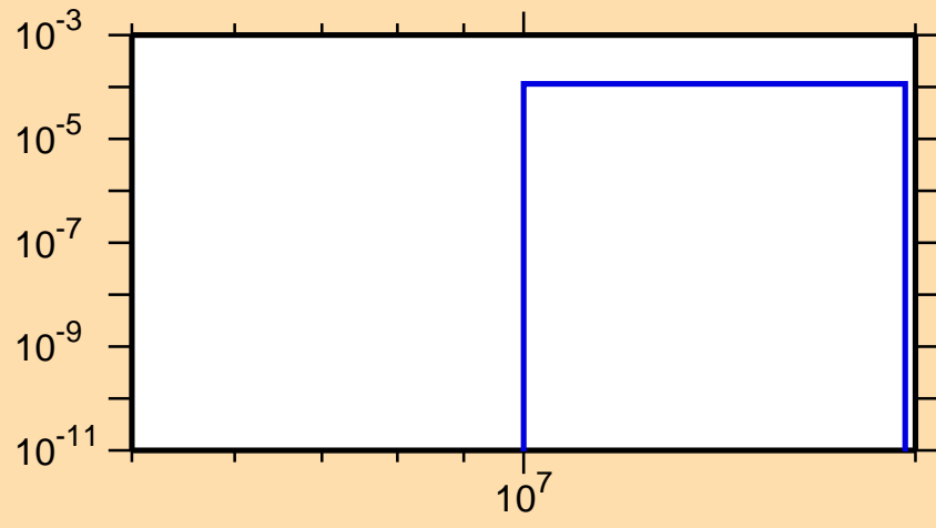
\sigma vs. E for ^{84}\text{Se}(n,p)
