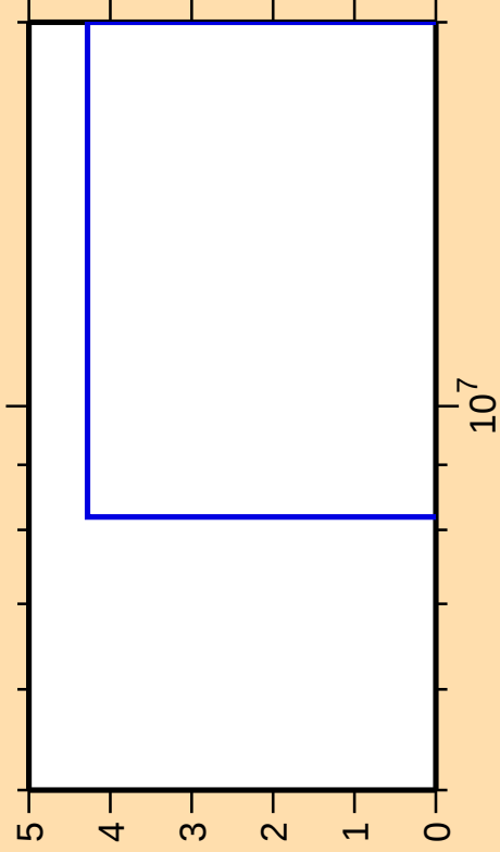
\Delta\sigma/\sigma vs. E for ^{84}\text{Se}(n,2n)
