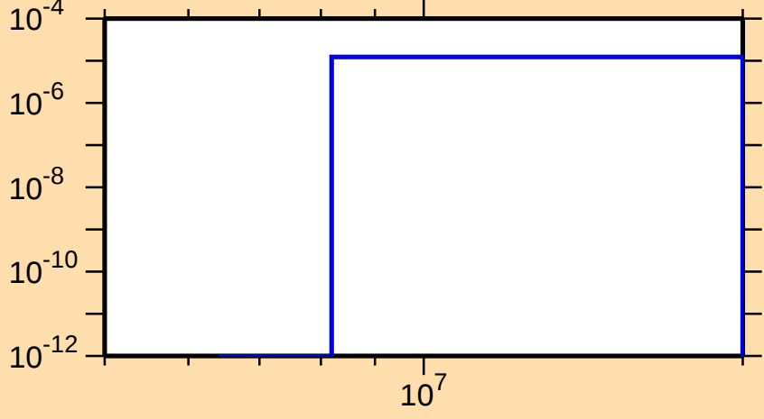
\sigma vs. E for ^{84}\text{Se}(n,\alpha)
