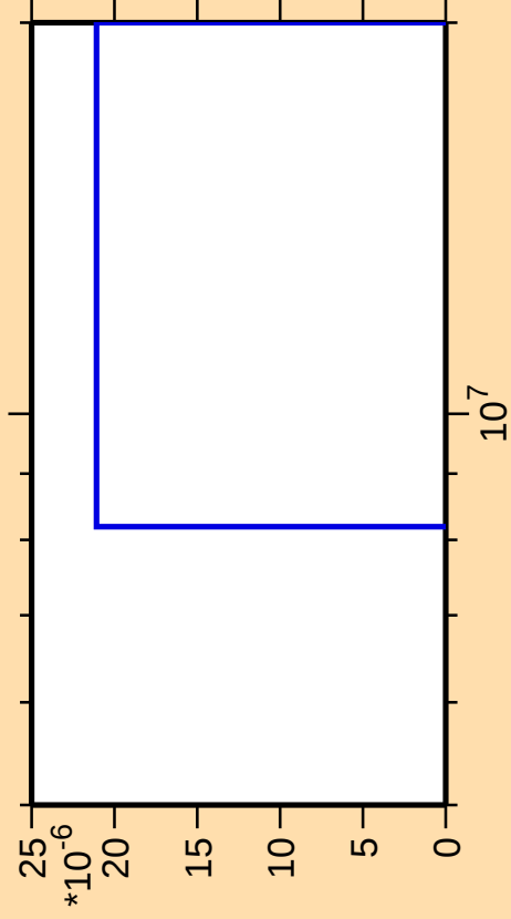
\Delta\sigma/\sigma vs. E for ^{84}\text{Se}(n,nt)
