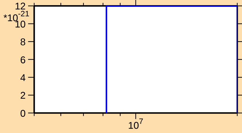
\sigma vs. E for ^{84}\text{Se}(n,\text{nd})
