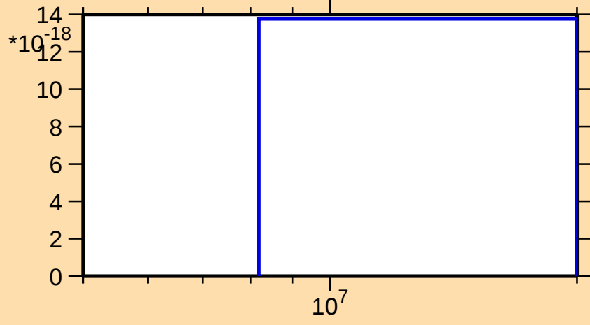
\sigma vs. E for ^{84}\text{Se}(n,nt)
