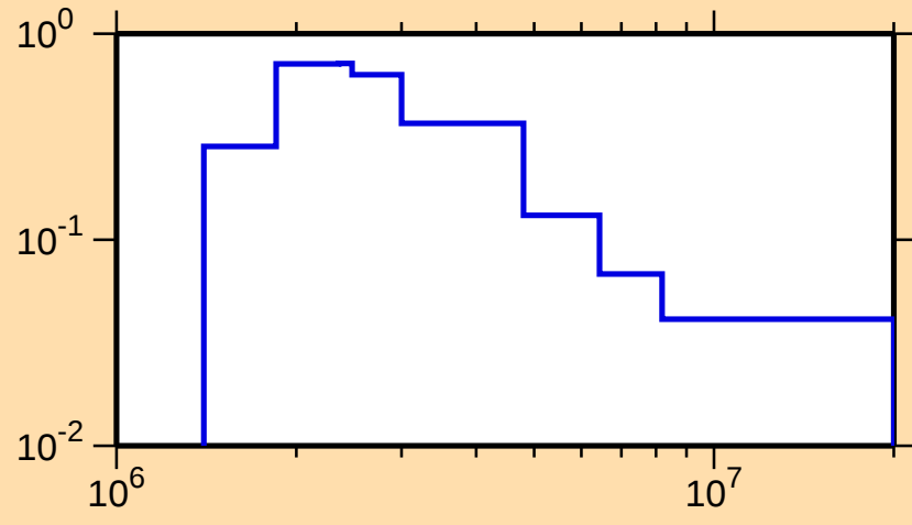
\sigma vs. E for ^{84}\text{Se}(n,n_1)
