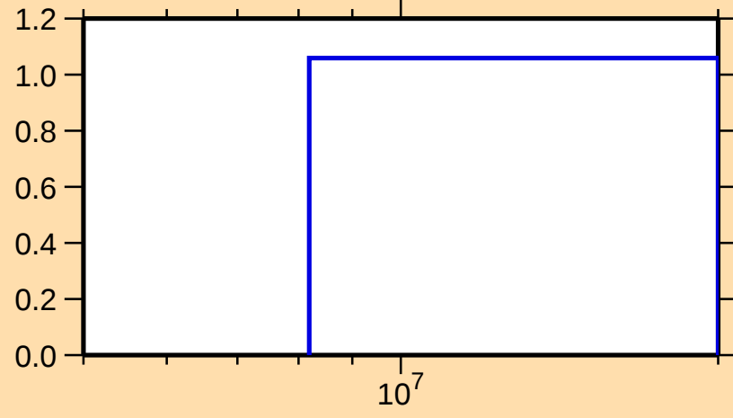
\sigma vs. E for ^{84}\text{Se}(n,2n)
