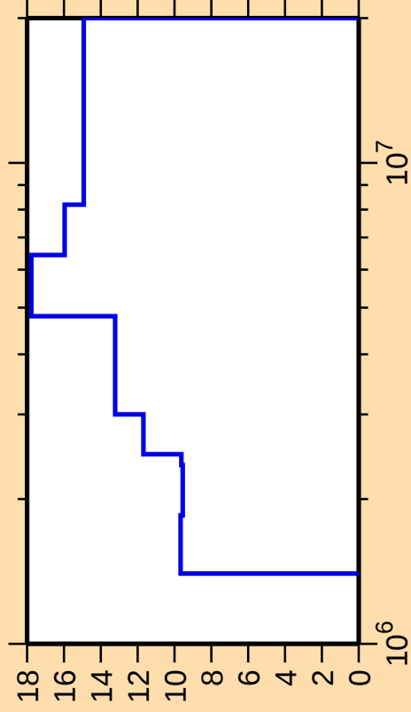
\Delta\sigma/\sigma vs. E for ^{84}\text{Se}(n,n_1)
