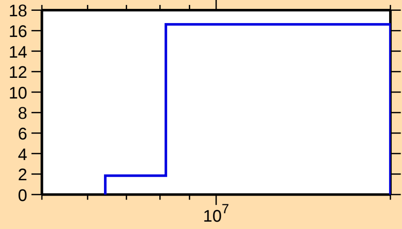
\Delta\sigma/\sigma vs. E for ^{84}\text{Se}(n,n\text{cont.})
