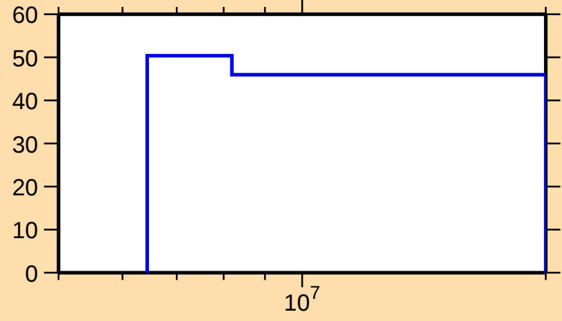
\Delta\sigma/\sigma vs. E for ^{84}\text{Se}(n,\gamma)
