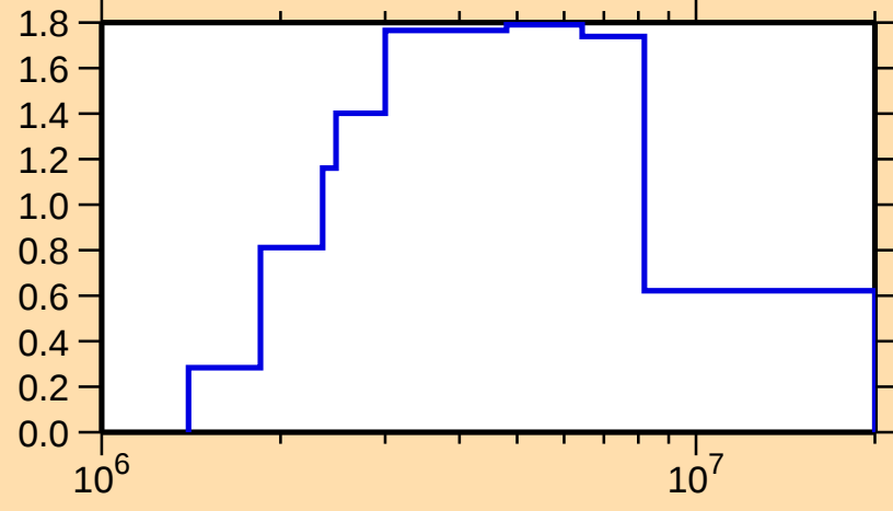
\sigma vs. E for ^{84}\text{Se}(n,\text{inel.})
