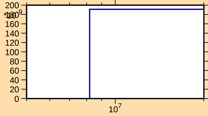
\sigma vs. E for ^{84}\text{Se}(n,n\alpha)
