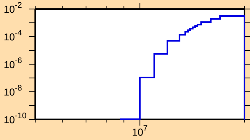
\sigma vs. E for ^{85}\text{Se}(n,p)
