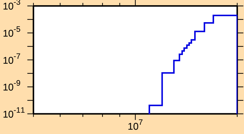
\sigma vs. E for ^{85}\text{Se}(n,t)
