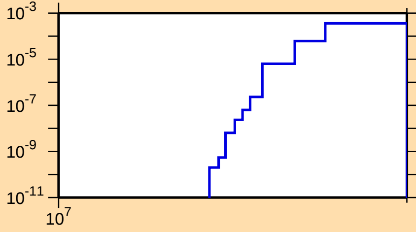
\sigma vs. E for ^{85}\text{Se}(n,d)
