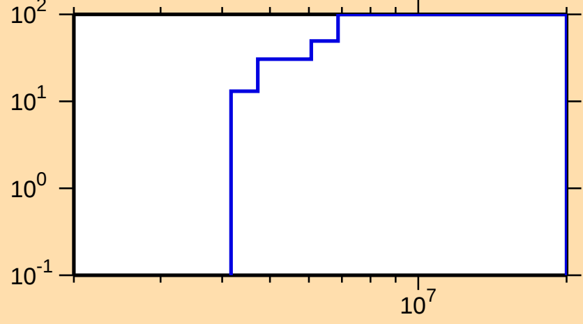
\Delta\sigma/\sigma vs. E for ^{85}\text{Se}(n,\text{inel.})
