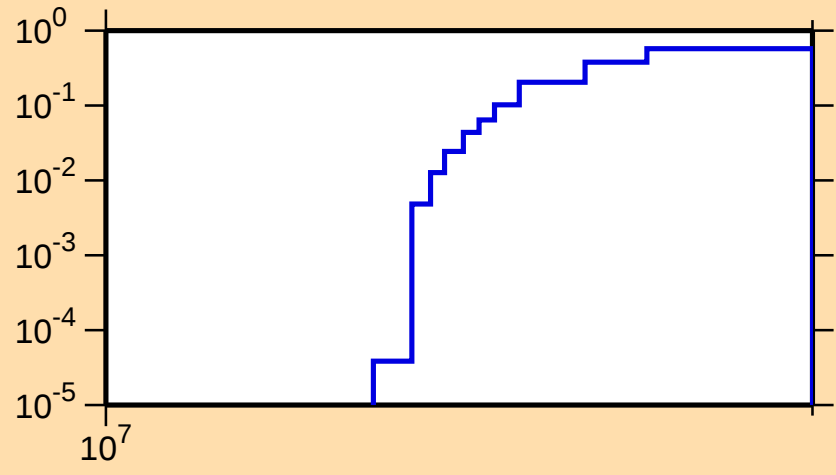
\sigma vs. E for ^{85}\text{Se}(n,3n)
