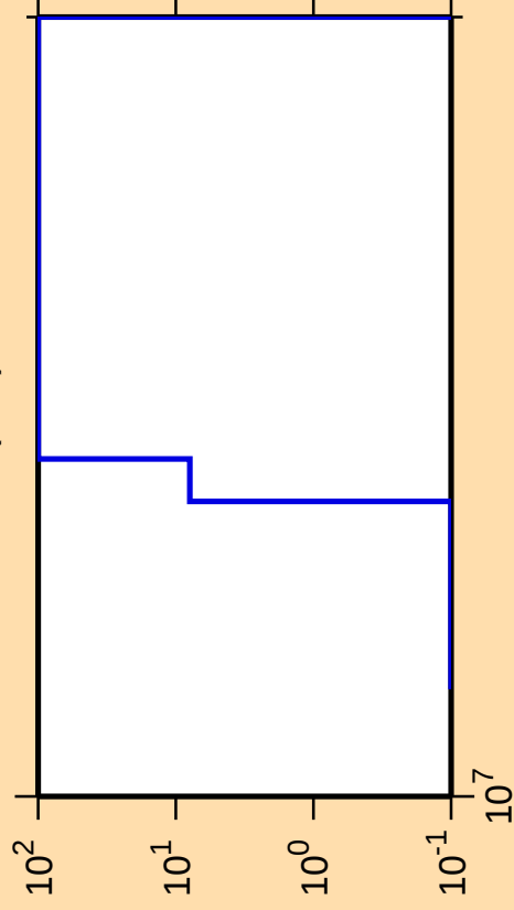
\Delta\sigma/\sigma vs. E for ^{85}\text{Se}(n,d)
