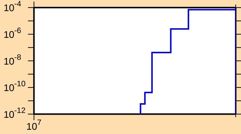
\sigma vs. E for ^{85}\text{Se}(n,np)
