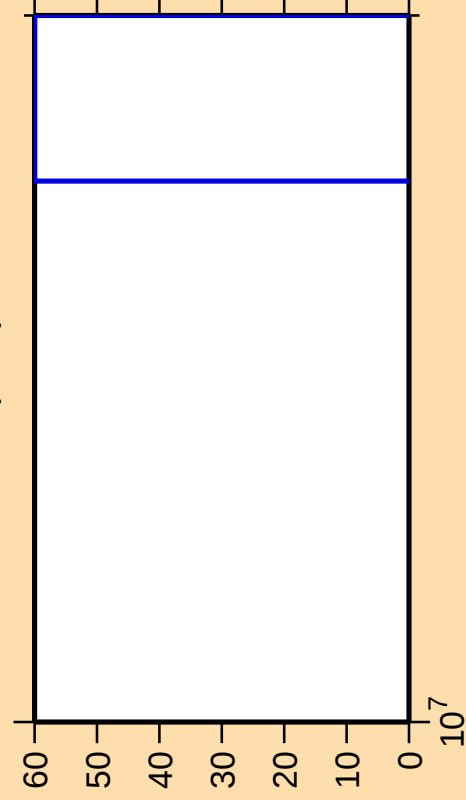
\Delta\sigma/\sigma vs. E for ^{85}\text{Se}(n,\text{nt})
