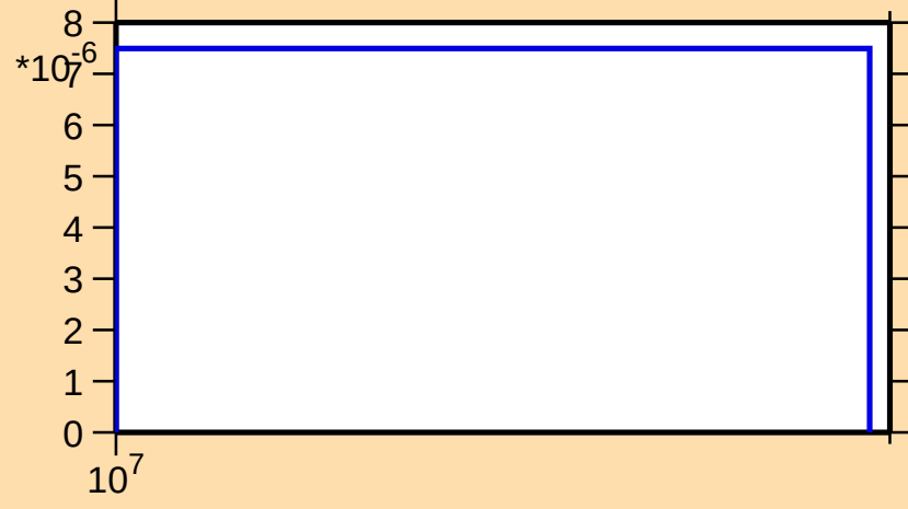
\sigma vs. E for ^{85}\text{Se}(n,d)
