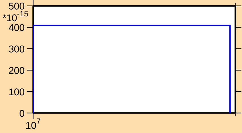
\sigma vs. E for ^{85}\text{Se}(n,\text{nt})
