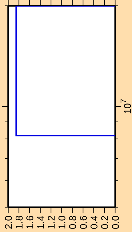
\Delta\sigma/\sigma vs. E for ^{85}\text{Se}(n,2n\alpha)
