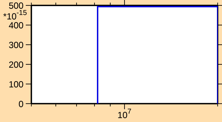
\sigma vs. E for ^{85}\text{Se}(n,2n\alpha)
