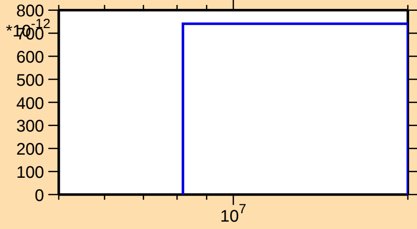
\sigma vs. E for ^{85}\text{Se}(n,\text{nd})
