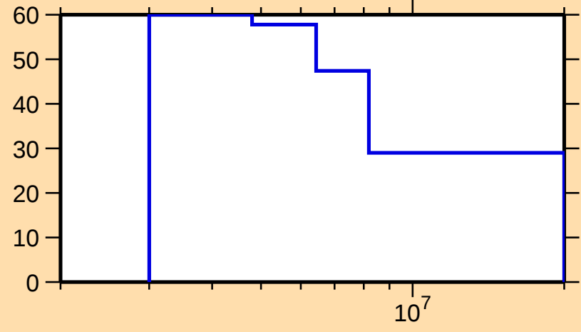
\Delta\sigma/\sigma vs. E for ^{85}\text{Se}(n,2n)
