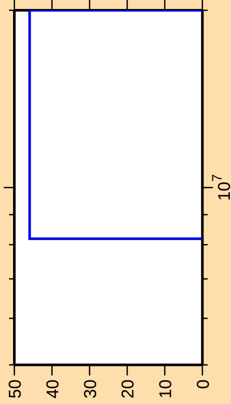
\Delta\sigma/\sigma vs. E for ^{85}\text{Se}(n,3n)
