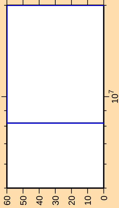
\Delta\sigma/\sigma vs. E for ^{85}\text{Se}(n,\text{nd})
