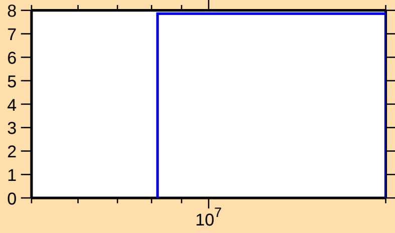
\Delta\sigma/\sigma vs. E for ^{85}\text{Se}(n,\text{tot.})
