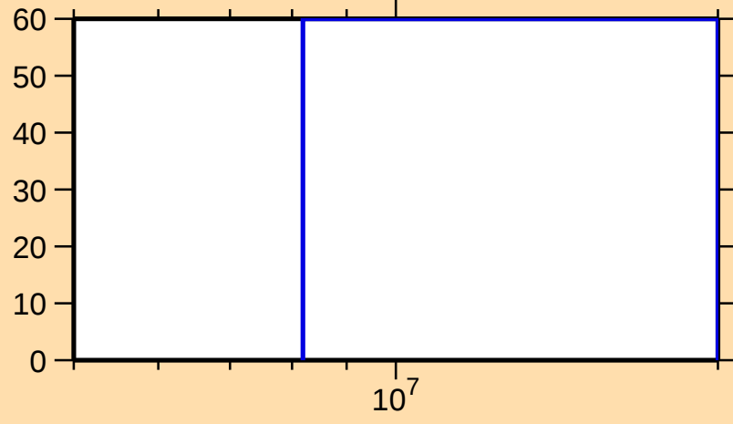
\Delta\sigma/\sigma vs. E for ^{85}\text{Se}(n,\text{inel.})
