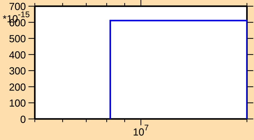
\sigma vs. E for ^{85}\text{Se}(n,nt)
