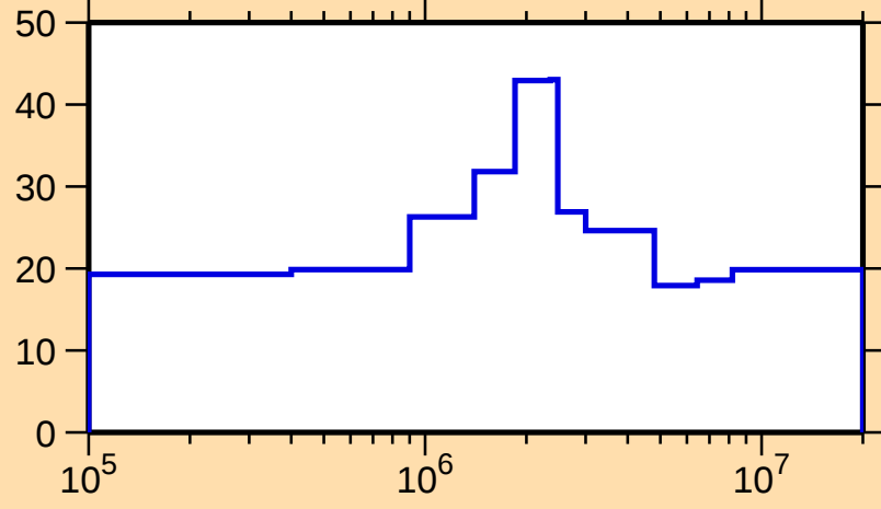
\Delta\sigma/\sigma vs. E for ^{85}\text{Se}(n,\text{el.})
