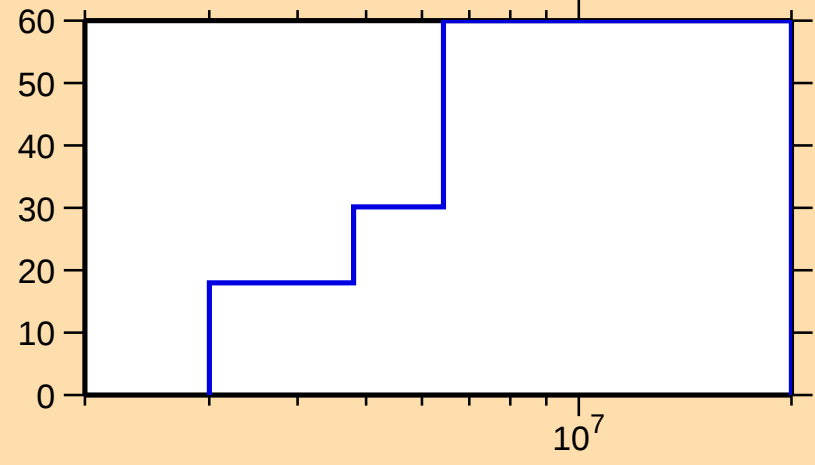
\Delta\sigma/\sigma vs. E for ^{85}\text{Se}(n,n\text{cont.})
