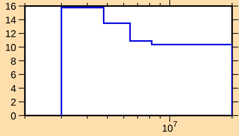
\Delta\sigma/\sigma vs. E for ^{85}\text{Se}(n,\text{nonel.})
