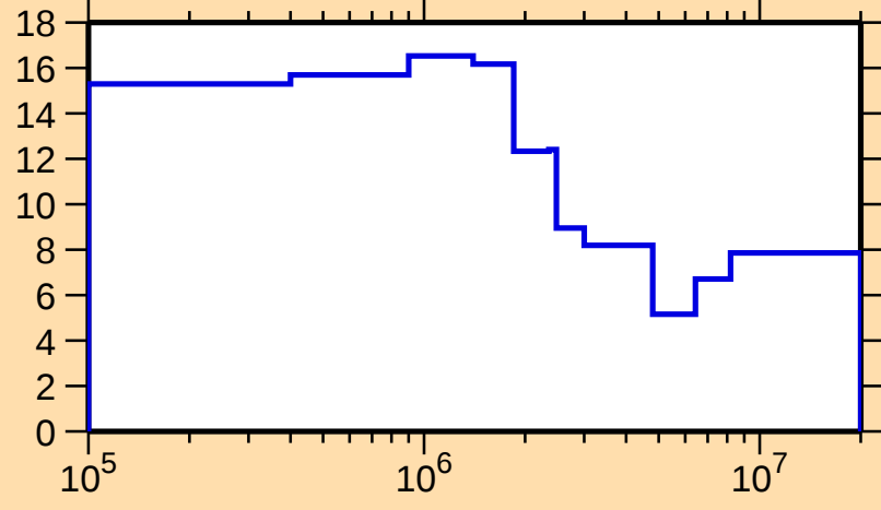
\Delta\sigma/\sigma vs. E for ^{85}\text{Se}(n,\text{tot.})
