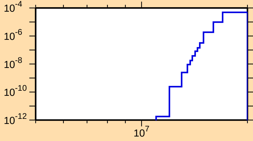
\sigma vs. E for ^{86}\text{Se}(n,n\alpha)
