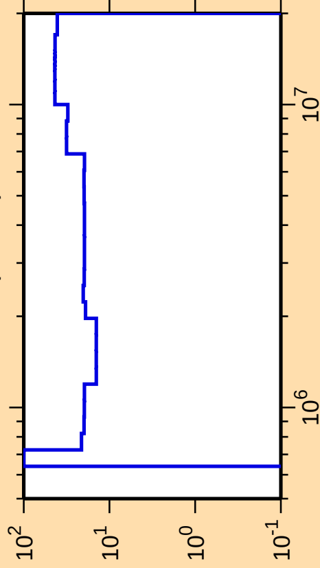
\Delta\sigma/\sigma vs. E for ^{86}\text{Se}(n,\text{inel.})
