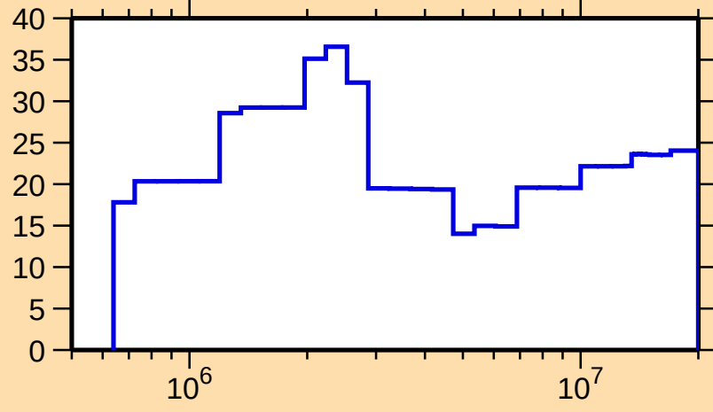
\Delta\sigma/\sigma vs. E for ^{86}\text{Se}(n,\text{el.})
