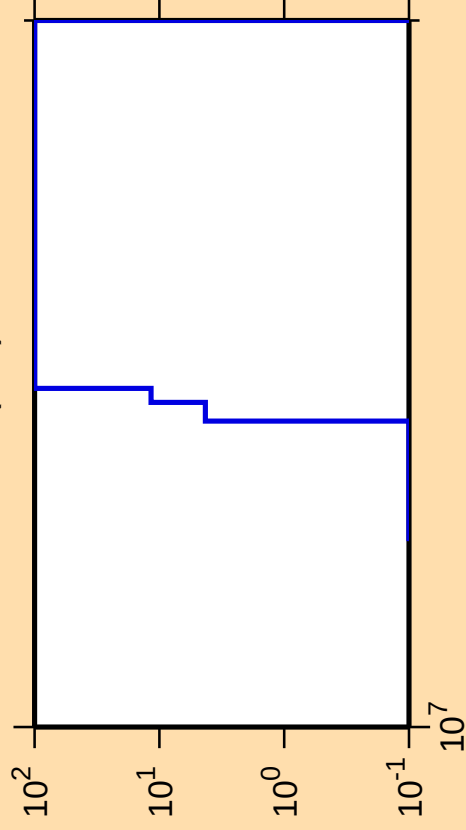
\Delta\sigma/\sigma vs. E for ^{86}\text{Se}(n,d)
