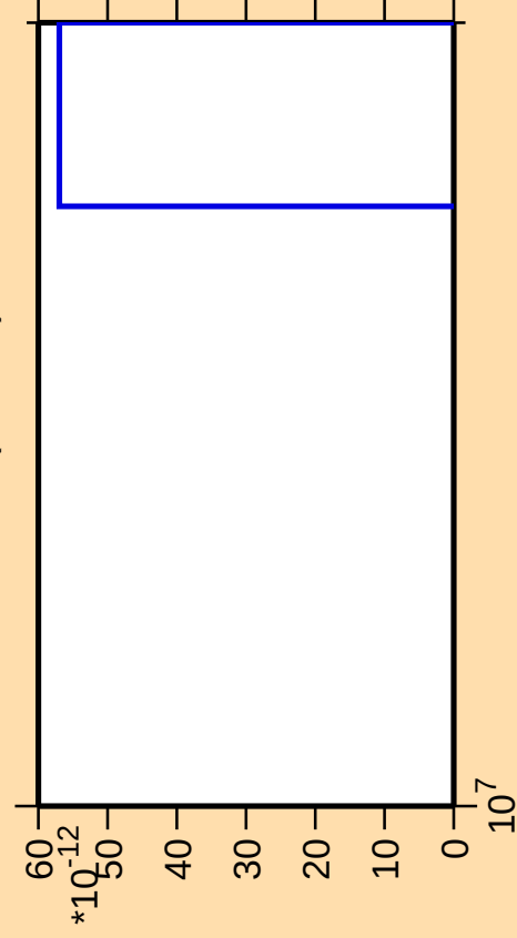
\Delta\sigma/\sigma vs. E for ^{86}\text{Se}(n,\text{He}3)
