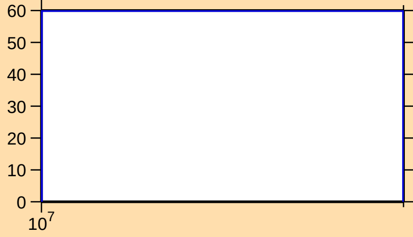
\Delta\sigma/\sigma vs. E for ^{86}\text{Se}(n,\gamma)
