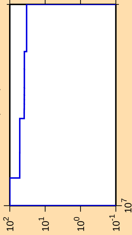
\Delta\sigma/\sigma vs. E for ^{86}\text{Se}(n,3n)
