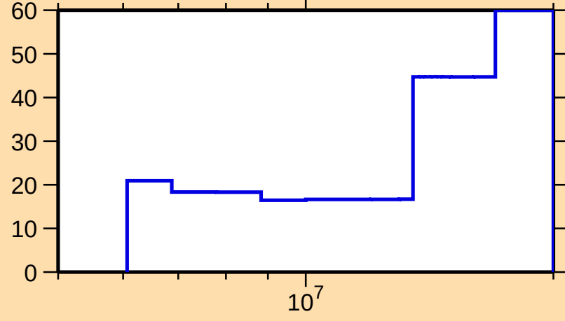
\Delta\sigma/\sigma vs. E for ^{86}\text{Se}(n,2n)
