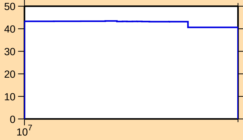
\Delta\sigma/\sigma vs. E for ^{86}\text{Se}(n,\text{inel.})
