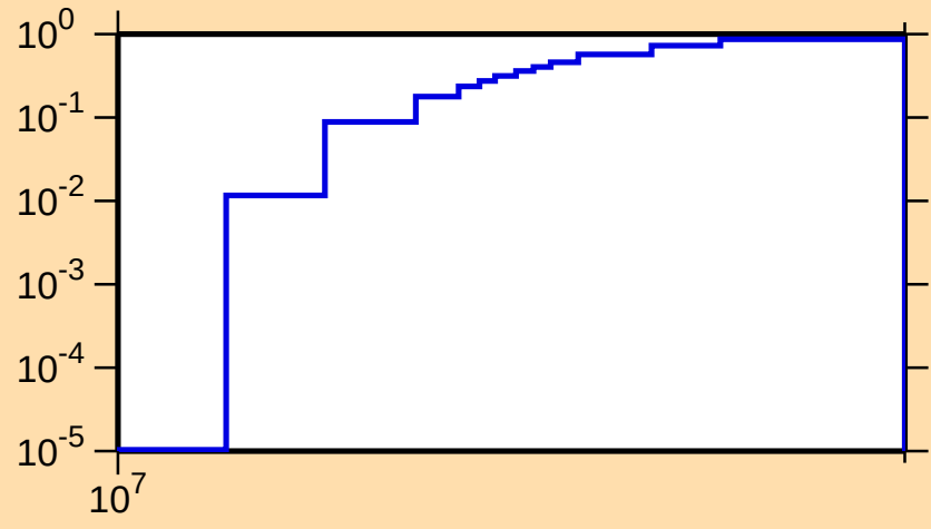
\sigma vs. E for ^{86}\text{Se}(n,3n)
