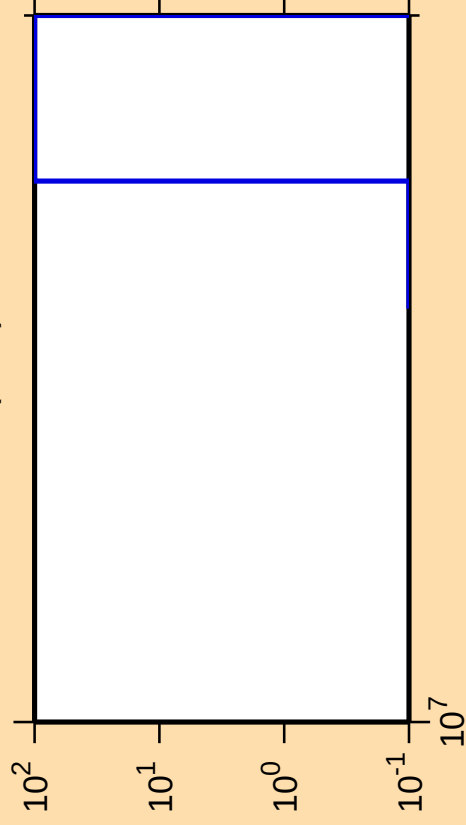
\Delta\sigma/\sigma vs. E for ^{86}\text{Se}(n,\text{nt})
