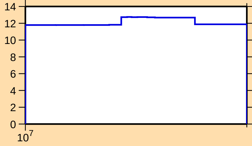
\Delta\sigma/\sigma vs. E for ^{86}\text{Se}(n,\text{nonel.})
