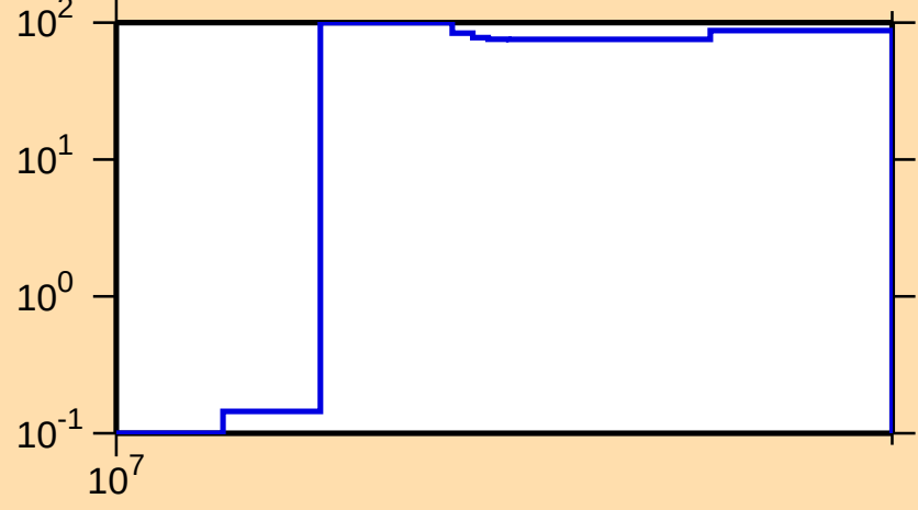
\Delta\sigma/\sigma vs. E for ^{86}\text{Se}(n,p)
