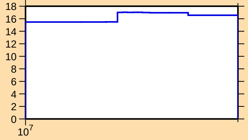
\Delta\sigma/\sigma vs. E for ^{86}\text{Se}(n,\text{tot.})
