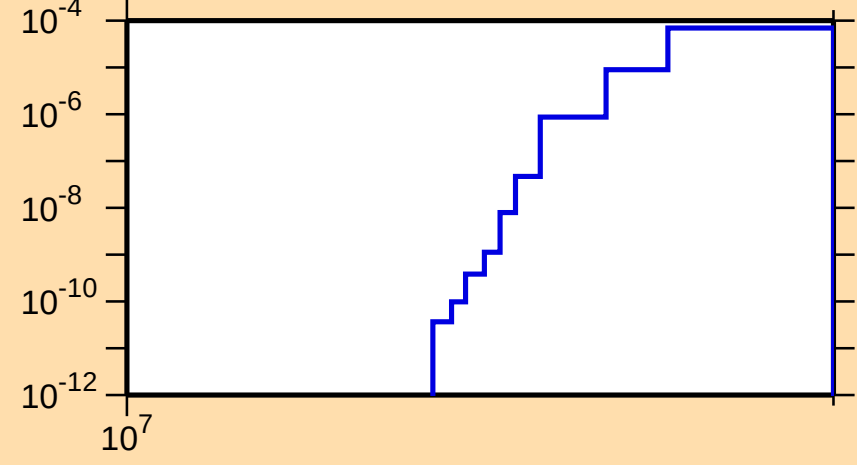
\sigma vs. E for ^{86}\text{Se}(n,t)
