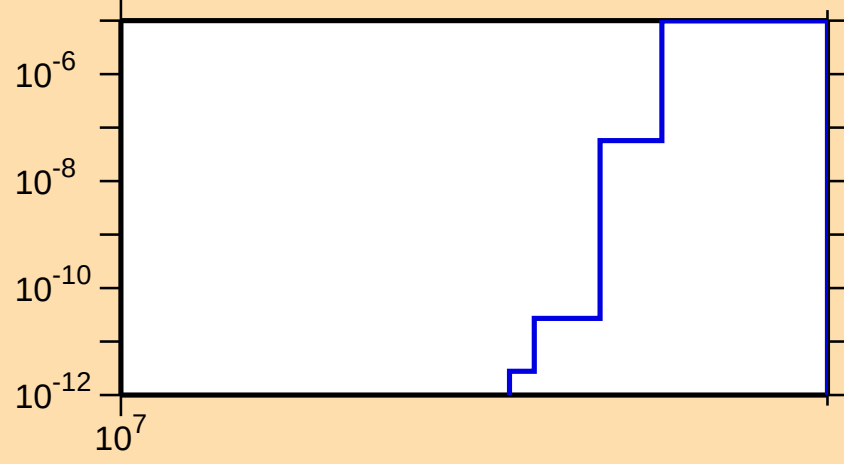
\sigma vs. E for ^{86}\text{Se}(n,np)
