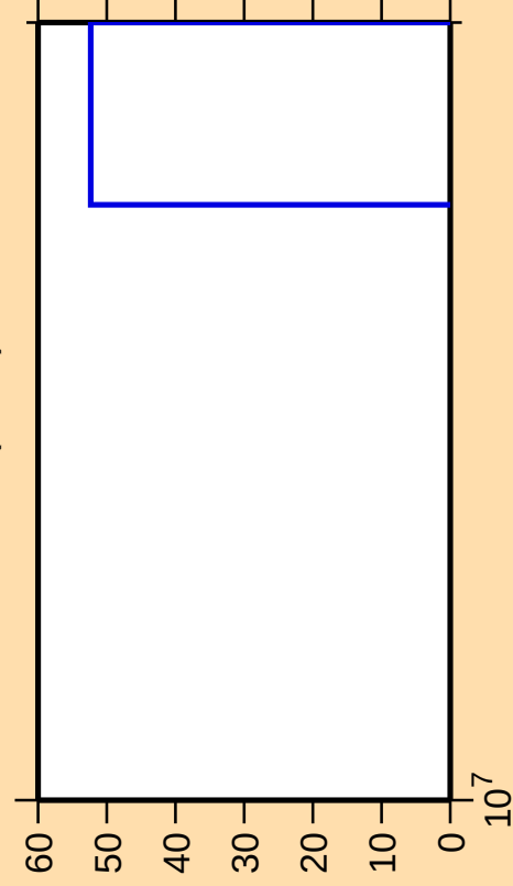
\Delta\sigma/\sigma vs. E for ^{86}\text{Se}(n,\text{nd})
