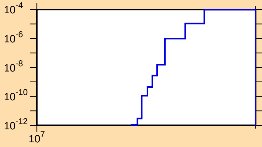
\sigma vs. E for ^{86}\text{Se}(n,d)
