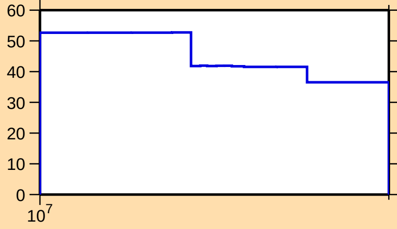
\Delta\sigma/\sigma vs. E for ^{86}\text{Se}(n,n_1)
