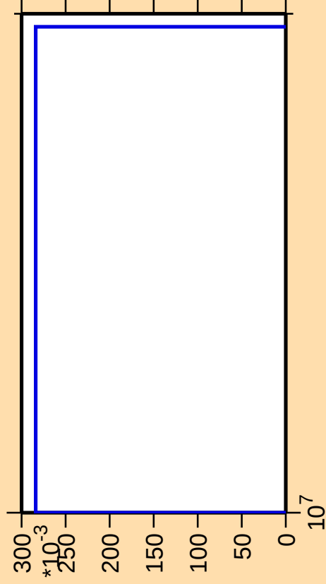
\Delta\sigma/\sigma vs. E for ^{86}\text{Se}(n,\text{nd})
