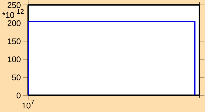
\sigma vs. E for ^{86}\text{Se}(n,\text{nt})
