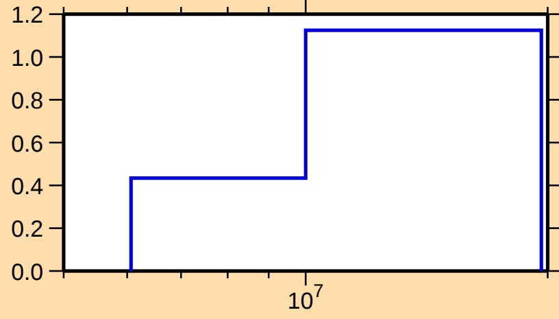
\sigma vs. E for ^{86}\text{Se}(n,2n)
