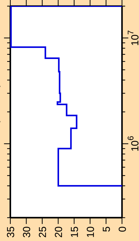
\Delta\sigma/\sigma vs. E for ^{86}\text{Se}(\text{n,inel.})
