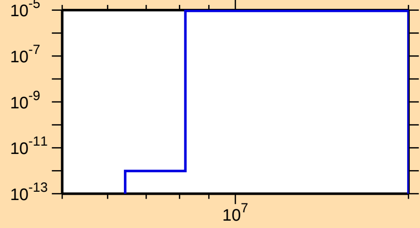
\sigma vs. E for ^{86}\text{Se}(n,\alpha)
