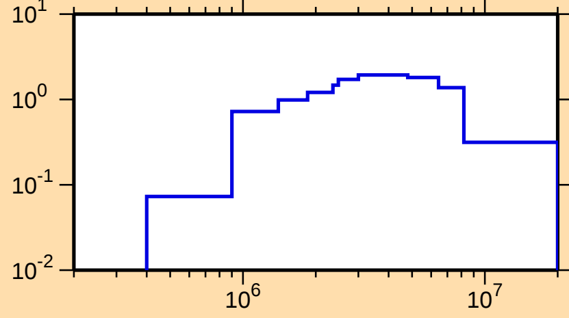
\sigma vs. E for ^{86}\text{Se}(n,\text{inel.})
