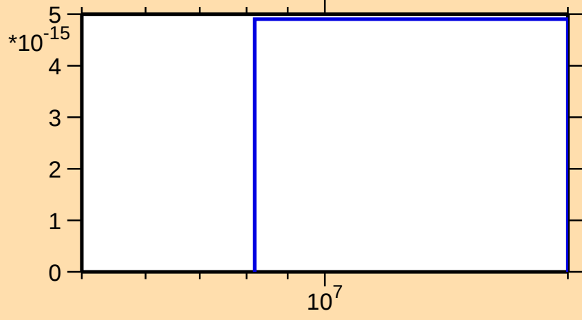
\sigma vs. E for ^{86}\text{Se}(n,2n\alpha)
