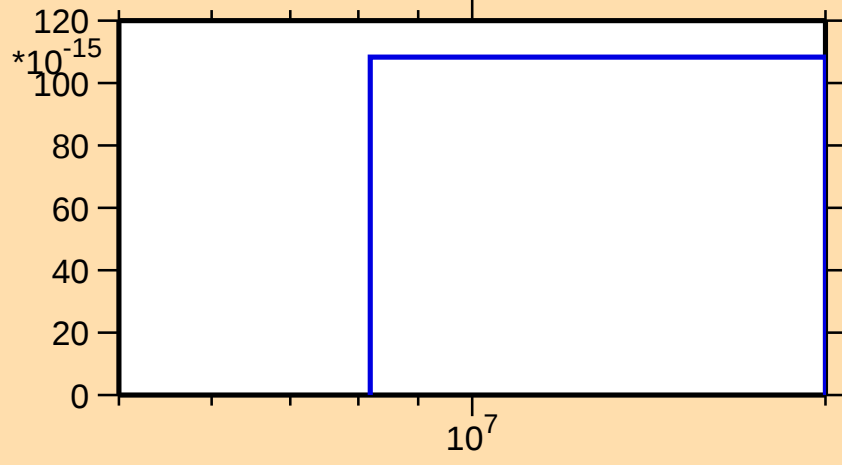
\sigma vs. E for ^{86}\text{Se}(n,\text{nd})
