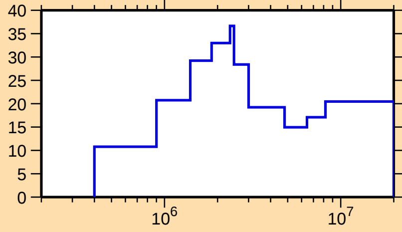
\Delta\sigma/\sigma vs. E for ^{86}\text{Se}(\text{n,el.})
