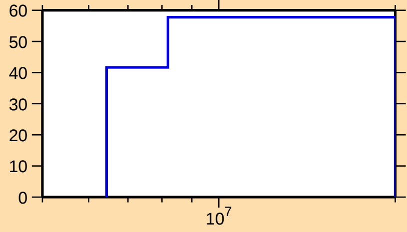
\Delta\sigma/\sigma vs. E for ^{86}\text{Se}(n,n\text{cont.})
