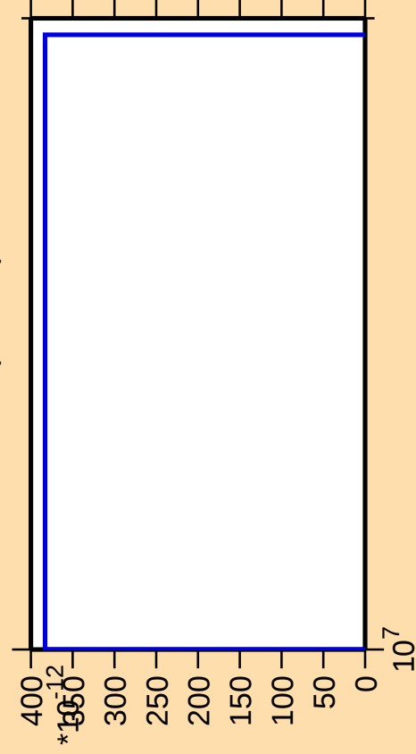
\Delta\sigma/\sigma vs. E for ^{87}\text{Se}(n,3n\alpha)
