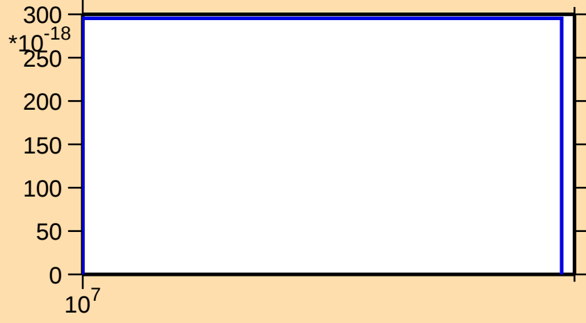
\sigma vs. E for ^{87}\text{Se}(n,2np)
