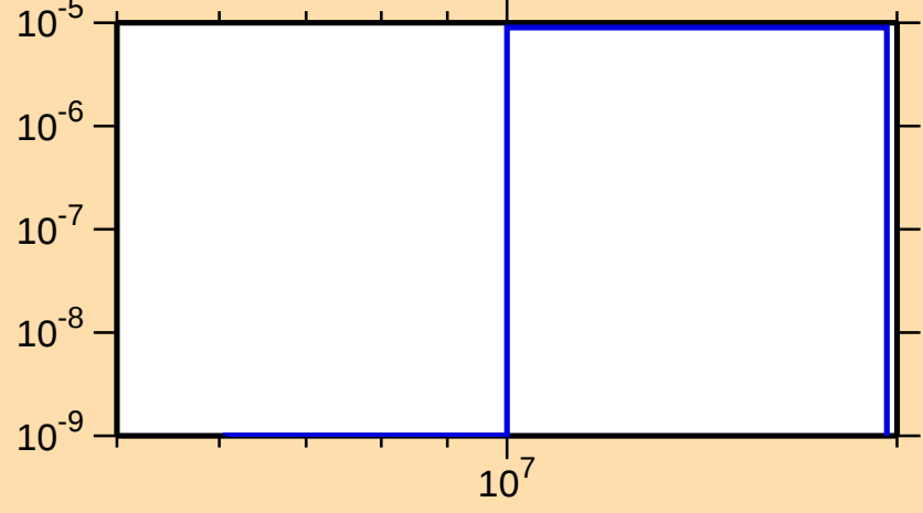
\sigma vs. E for ^{87}\text{Se}(n,\alpha)
