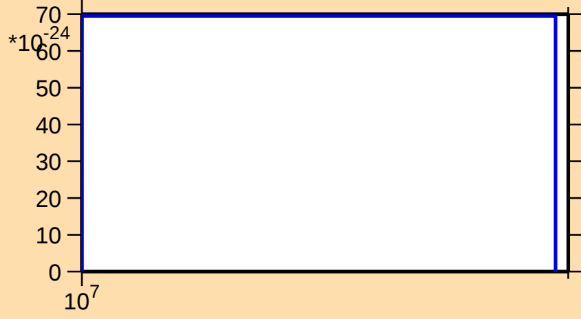
\sigma vs. E for ^{87}\text{Se}(n,3n\alpha)
