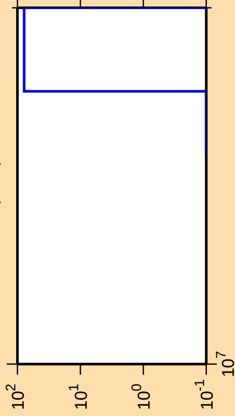
\Delta\sigma/\sigma vs. E for ^{88}\text{Se}(n,\text{nt})
