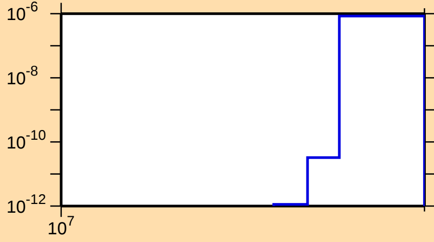
\sigma vs. E for ^{88}\text{Se}(n,np)
