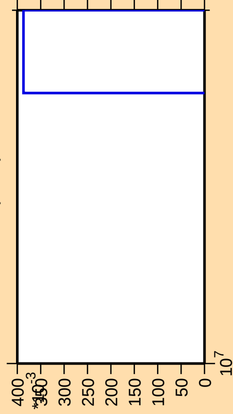
\Delta\sigma/\sigma vs. E for ^{88}\text{Se}(n,\text{nd})
