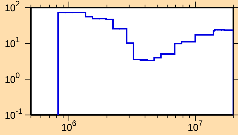
\Delta\sigma/\sigma vs. E for ^{88}\text{Se}(\text{n,el.})
