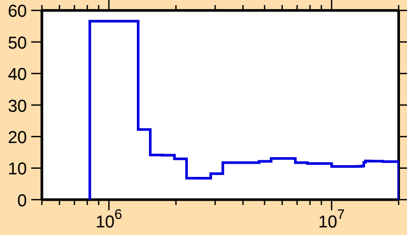
\Delta\sigma/\sigma vs. E for ^{88}\text{Se}(\text{n,nonel.})
