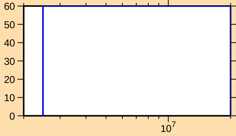
\Delta\sigma/\sigma vs. E for ^{88}\text{Se}(n,n_1)
