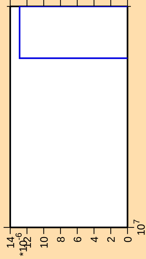
\Delta\sigma/\sigma vs. E for ^{30}\text{Si}(n,p\alpha)
