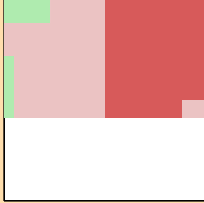
\Delta\sigma/\sigma vs. E for ^{30}\text{Si}(n,\text{el.})
