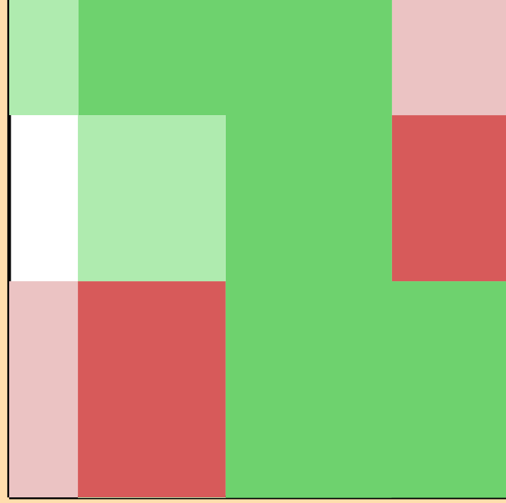
\Delta\sigma/\sigma vs. E for ^{30}\text{Si}(n,2n)
