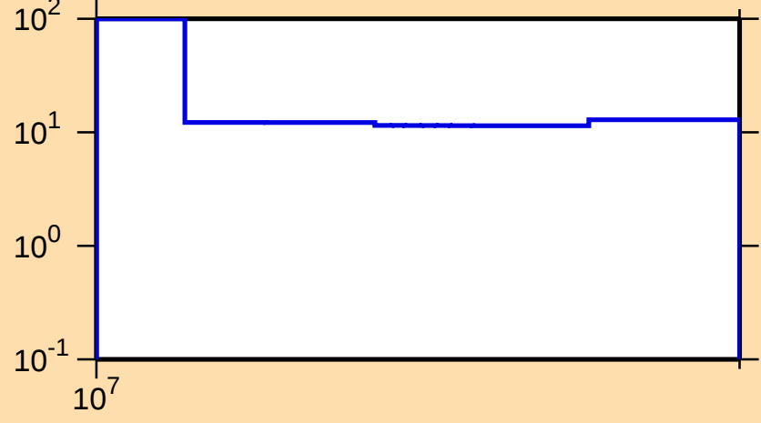
\Delta\sigma/\sigma vs. E for ^{30}\text{Si}(n,2n)
