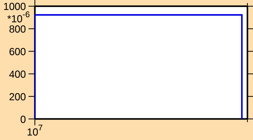
\sigma vs. E for ^{30}\text{Si}(n,np)
