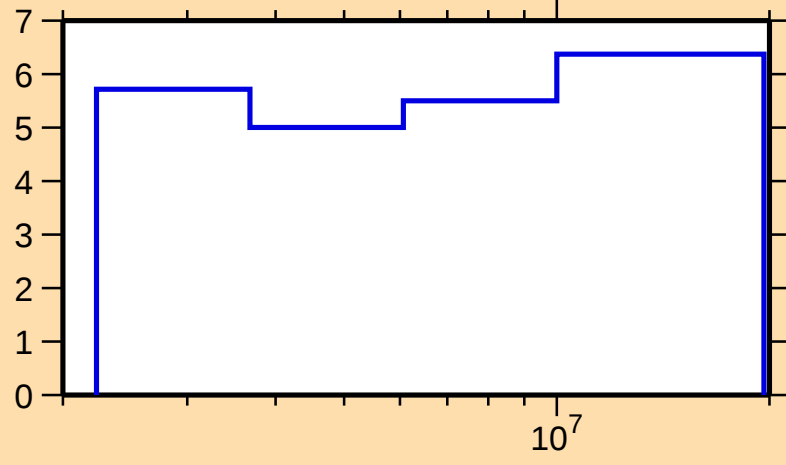
\Delta\sigma/\sigma vs. E for ^{30}\text{Si}(\text{n,nonel.})
