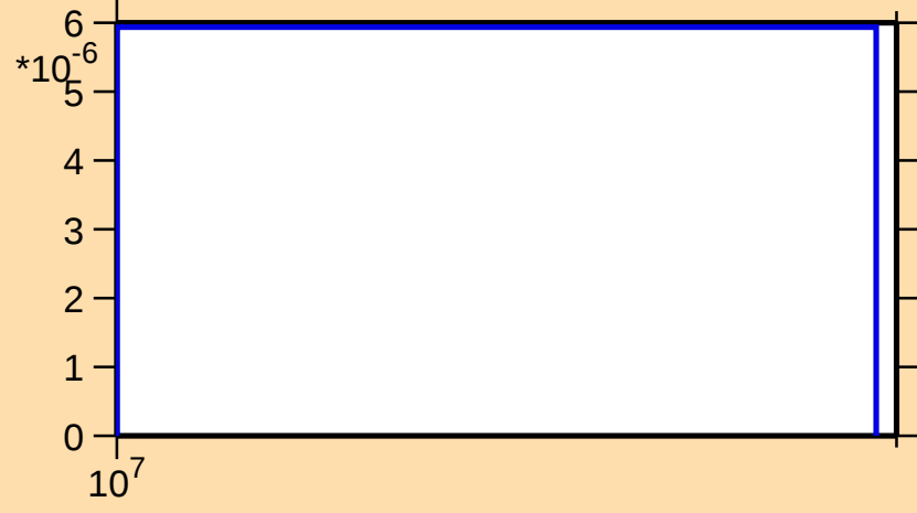
\sigma vs. E for ^{30}\text{Si}(n,t)
