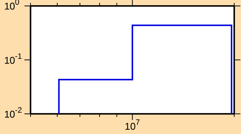
\sigma vs. E for ^{30}\text{Si}(n,n\text{cont.})
