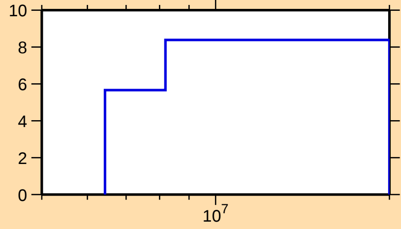
\Delta\sigma/\sigma vs. E for ^{30}\text{Si}(\text{n},\text{inel.})
