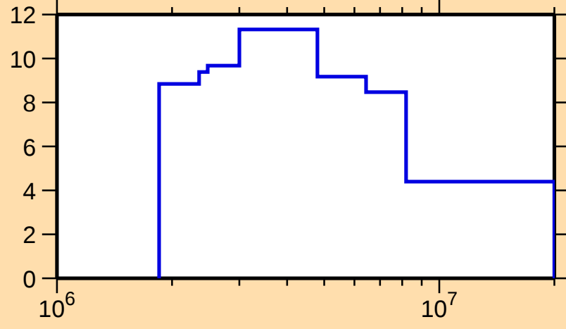
\Delta\sigma/\sigma vs. E for ^{30}\text{Si}(\text{n,tot.})
