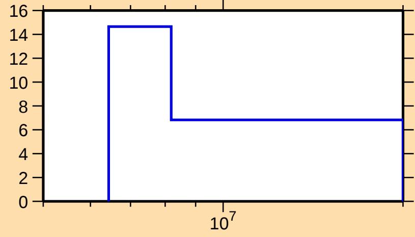
\Delta\sigma/\sigma vs. E for ^{30}\text{Si}(\text{n},\text{el.})
