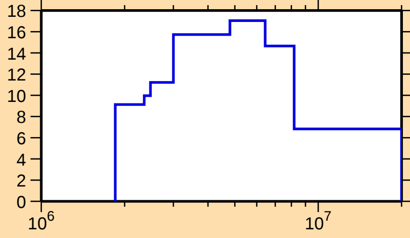
\Delta\sigma/\sigma vs. E for ^{30}\text{Si}(\text{n,el.})
