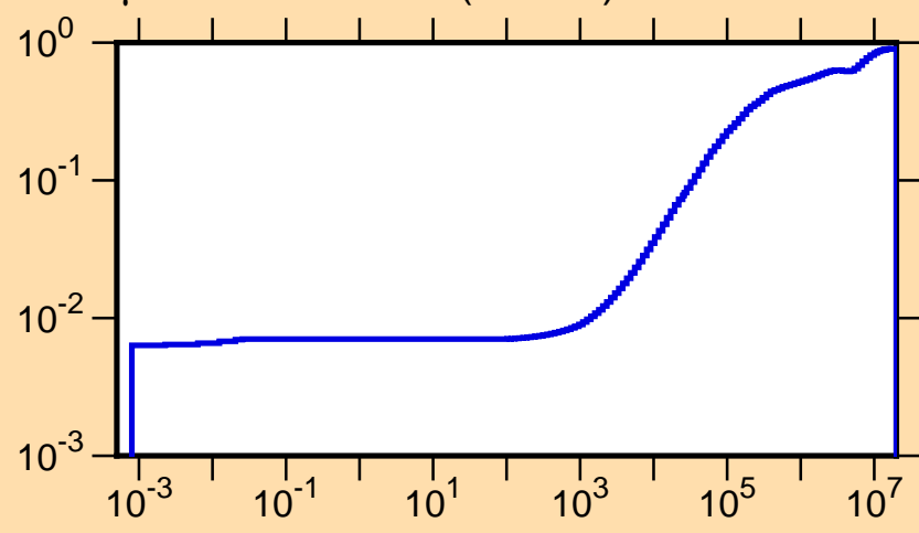
\mu vs. E for ^{107}\text{Sn}(\text{mt251})
