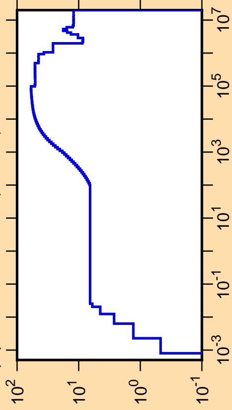
\Delta\mu/\mu vs. E for ^{107}\text{Sn}(\text{mt251})
