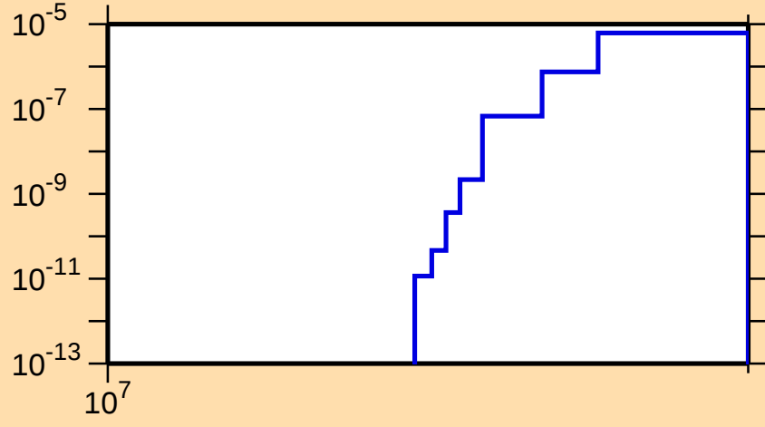
\sigma vs. E for ^{107}\text{Sn}(n,2n\alpha)
