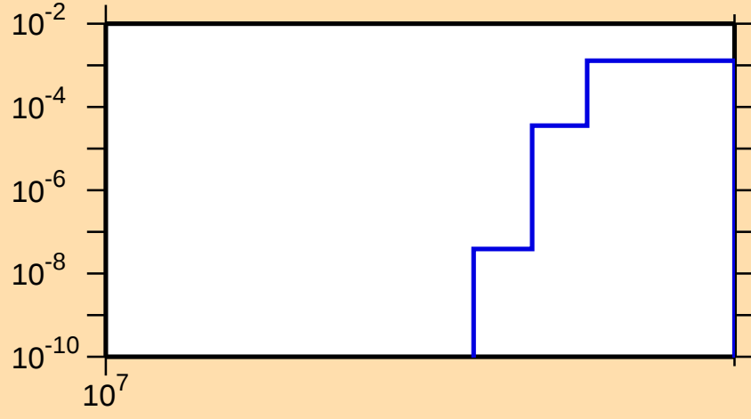
\sigma vs. E for ^{107}\text{Sn}(n,2np)
