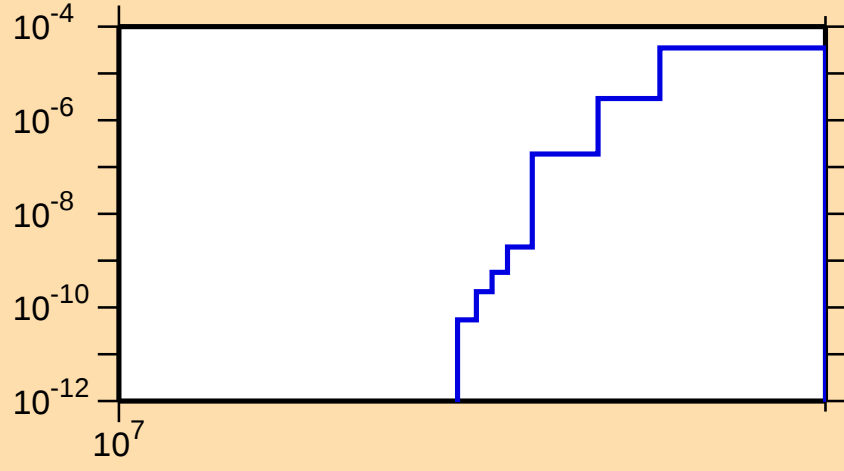
\sigma vs. E for ^{107}\text{Sn}(n,\text{nd})
