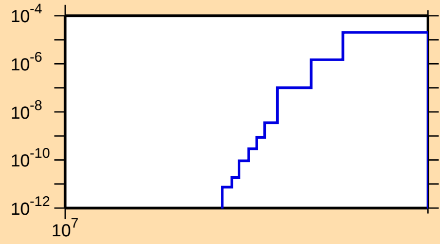
\sigma vs. E for ^{107}\text{Sn}(n,\text{pt})
