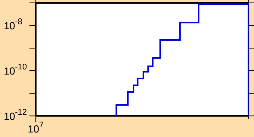
\sigma vs. E for ^{107}\text{Sn}(\text{mt117})
