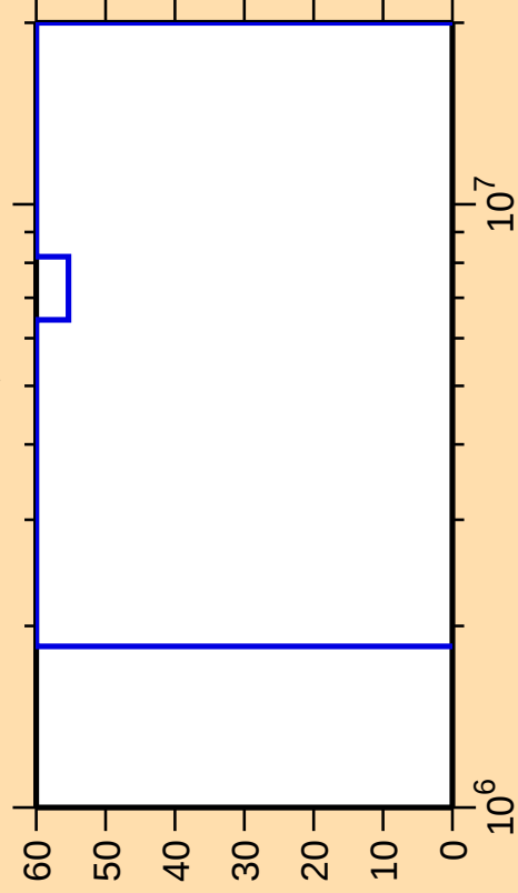
\Delta\sigma/\sigma vs. E for ^{107}\text{Sn}(n,\gamma)
