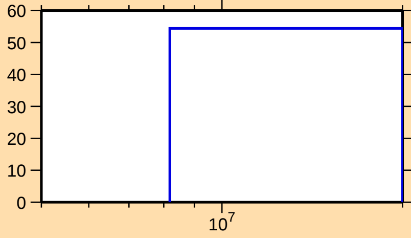
\Delta\sigma/\sigma vs. E for ^{107}\text{Sn}(n,\text{inel.})
