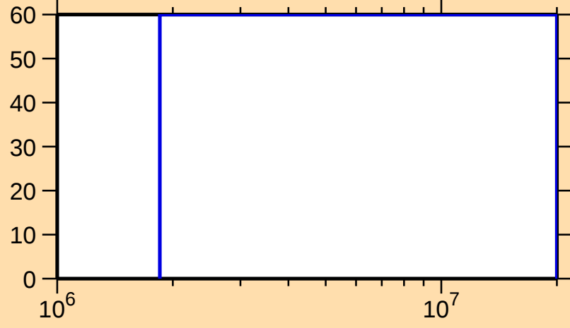
\Delta\sigma/\sigma vs. E for ^{107}\text{Sn}(n,n\text{cont.})
