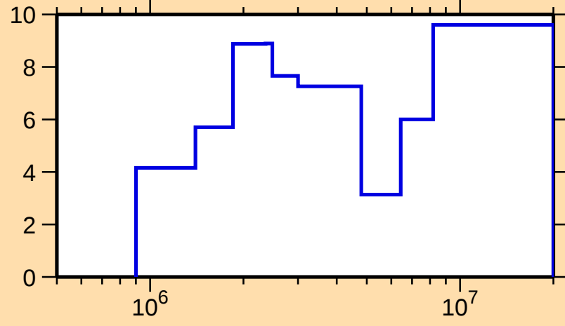
\Delta\sigma/\sigma vs. E for ^{114}\text{Sn}(n,\text{el.})
