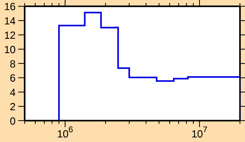
\Delta\sigma/\sigma vs. E for ^{114}\text{Sn}(n,\text{nonel.})
