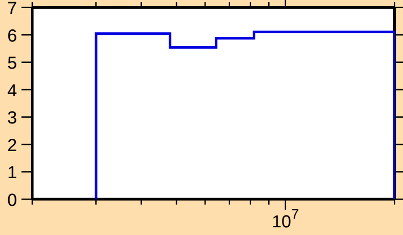
\Delta\sigma/\sigma vs. E for ^{114}\text{Sn}(n,n\text{onel.})
