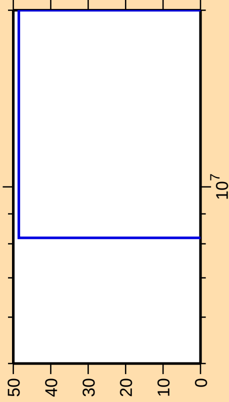
\Delta\sigma/\sigma vs. E for ^{114}\text{Sn}(n,3n)
