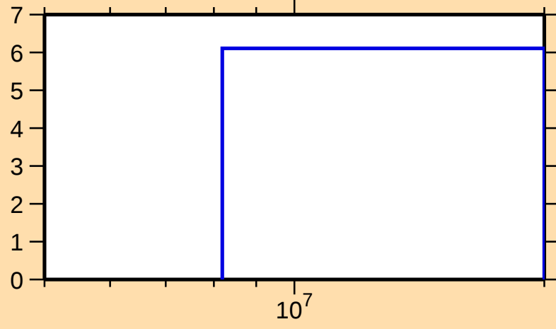
\Delta\sigma/\sigma vs. E for ^{114}\text{Sn}(n,\text{nonel.})
