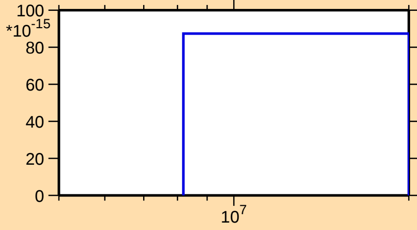
\sigma vs. E for ^{114}\text{Sn}(n,2np)
