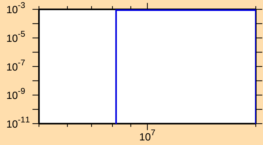
\sigma vs. E for ^{114}\text{Sn}(n,d)
