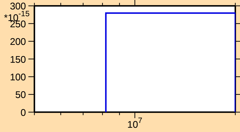
\sigma vs. E for ^{114}\text{Sn}(n,\text{pd})
