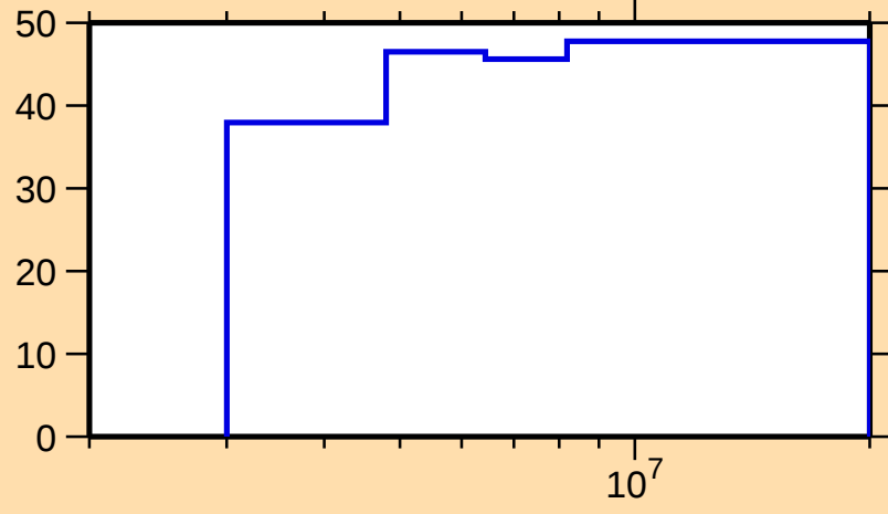
\Delta\sigma/\sigma vs. E for ^{114}\text{Sn}(n, n_1)
