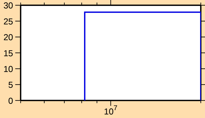
\Delta\sigma/\sigma vs. E for ^{114}\text{Sn}(n,\text{inel.})
