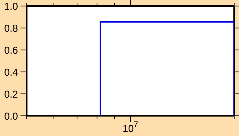
\sigma vs. E for ^{114}\text{Sn}(n,2n)
