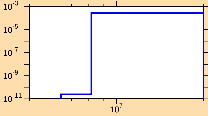
\sigma vs. E for ^{114}\text{Sn}(n,n\alpha)
