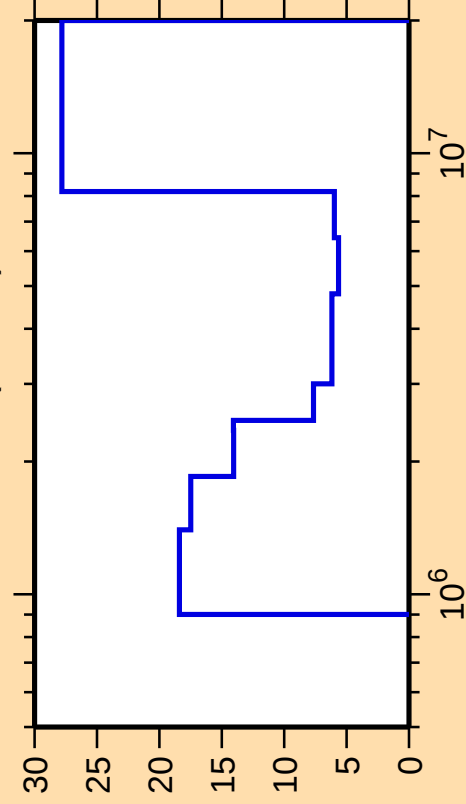
\Delta\sigma/\sigma vs. E for ^{114}\text{Sn}(n,\text{inel.})
