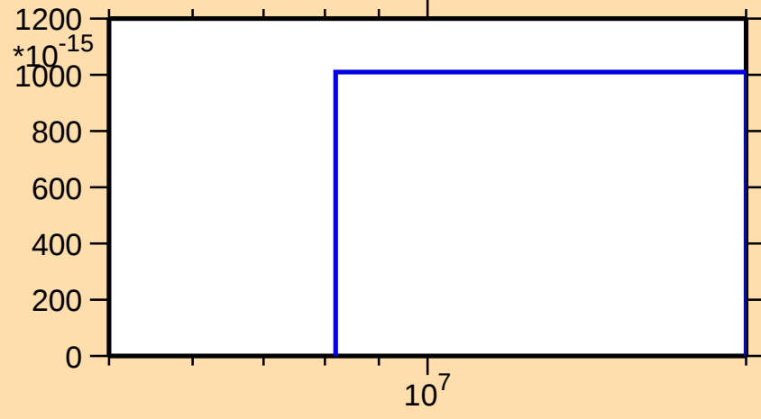
\sigma vs. E for ^{114}\text{Sn}(n,2n\alpha)
