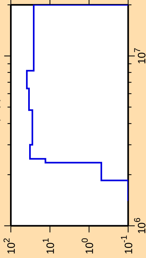
\Delta\sigma/\sigma vs. E for ^{114}\text{Sn}(n,p)
