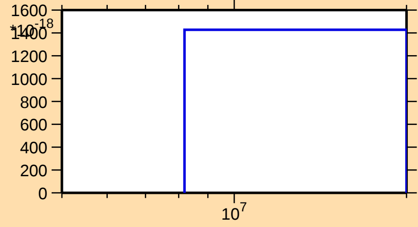
\sigma vs. E for ^{114}\text{Sn}(n,nt)
