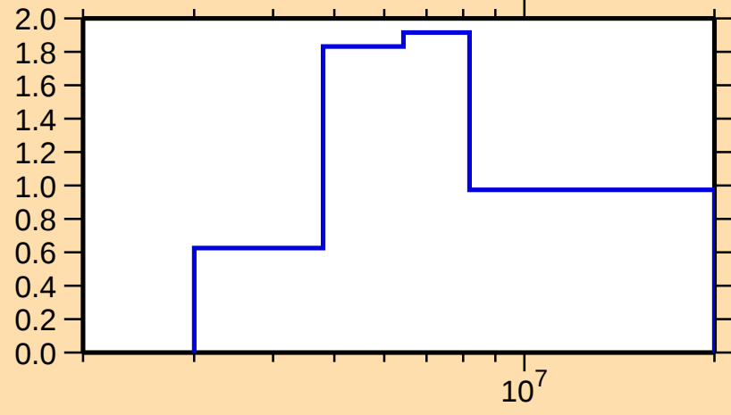
\sigma vs. E for ^{114}\text{Sn}(n,n\text{cont.})
