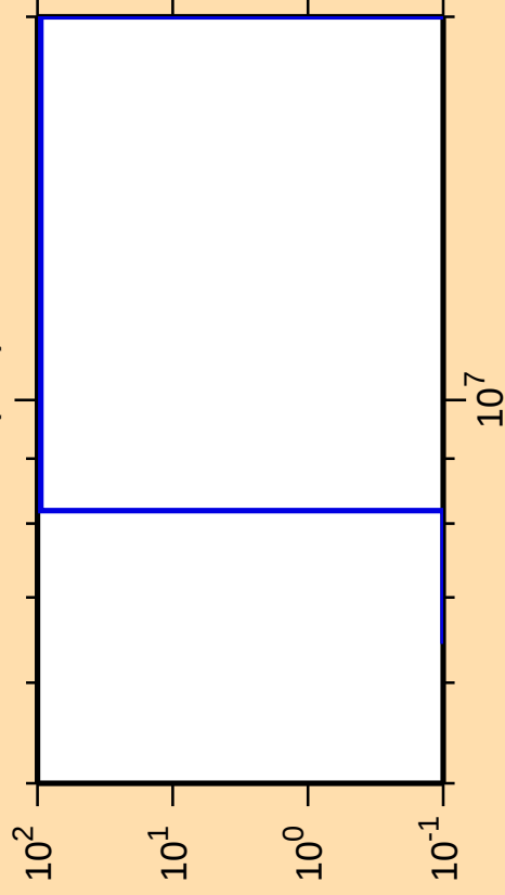
\Delta\sigma/\sigma vs. E for ^{114}\text{Sn}(n,d)
