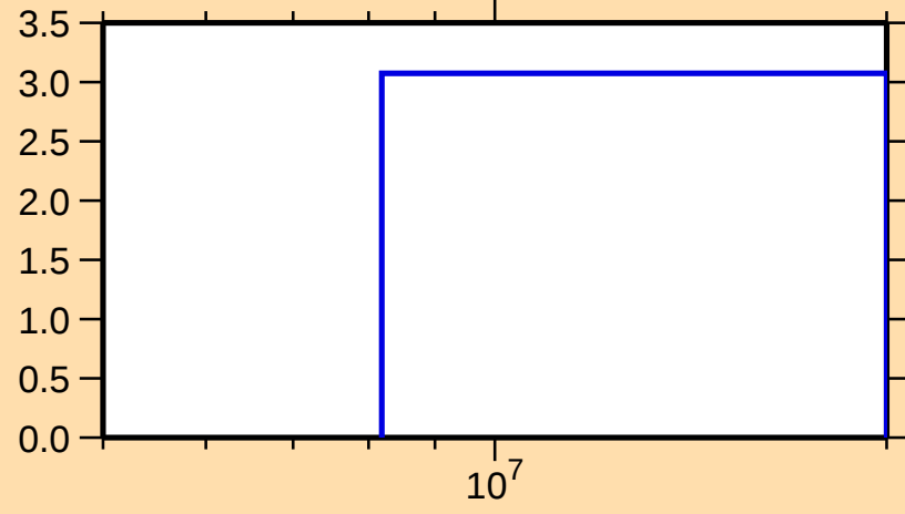
\Delta\sigma/\sigma vs. E for ^{114}\text{Sn}(n,\text{tot.})
