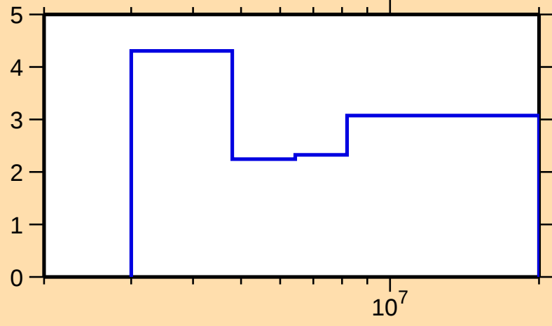
\Delta\sigma/\sigma vs. E for ^{114}\text{Sn}(n,\text{tot.})
