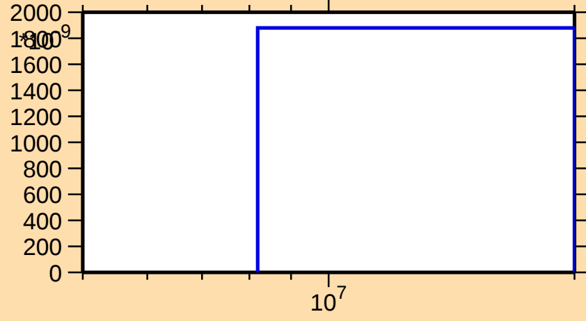
\sigma vs. E for ^{114}\text{Sn}(n,3n)
