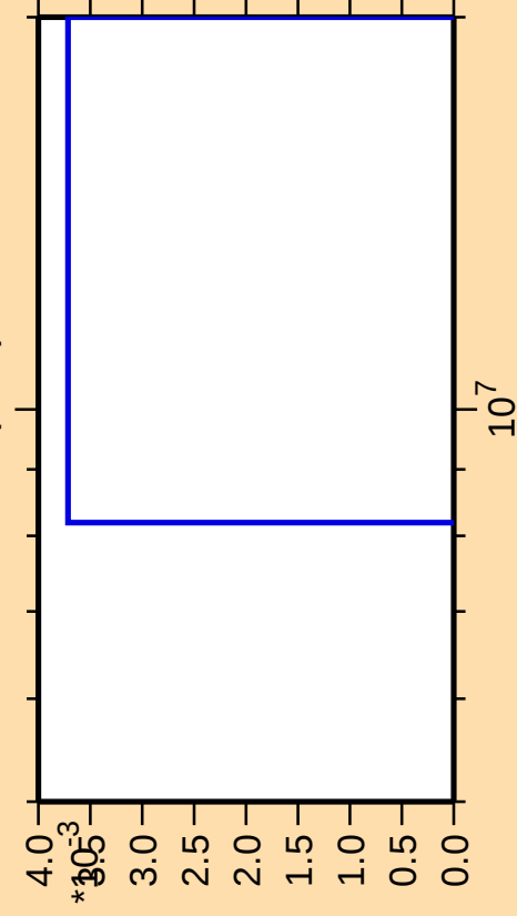
\Delta\sigma/\sigma vs. E for ^{114}\text{Sn}(n,nt)
