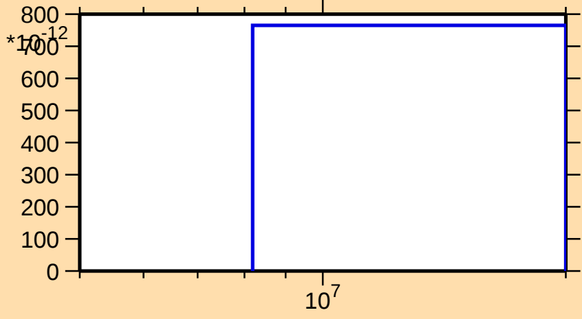
\sigma vs. E for ^{114}\text{Sn}(n,\text{He}3)
