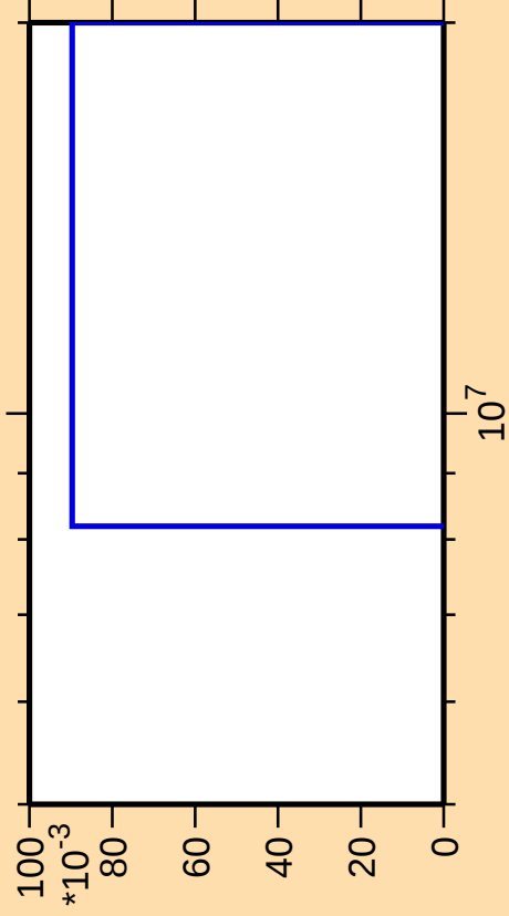
\Delta\sigma/\sigma vs. E for ^{114}\text{Sn}(n,2np)
