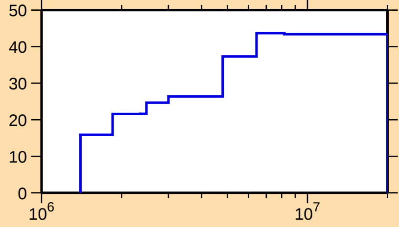
\Delta\sigma/\sigma vs. E for ^{114}\text{Sn}(n,\gamma)
