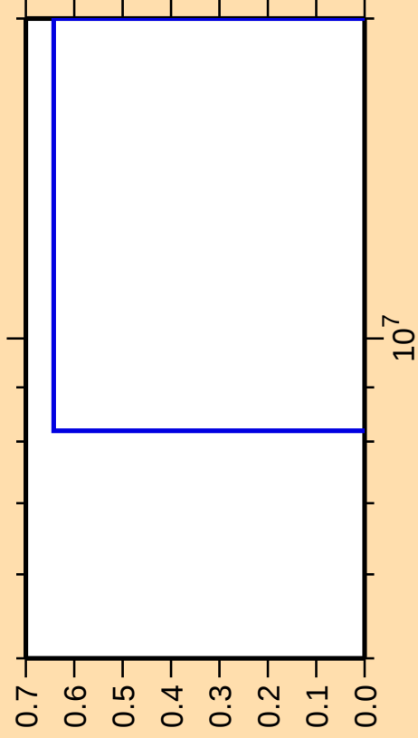
\Delta\sigma/\sigma vs. E for ^{114}\text{Sn}(n,\text{pd})
