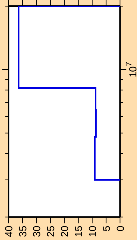
\Delta\sigma/\sigma vs. E for ^{114}\text{Sn}(n,n\text{cont.})
