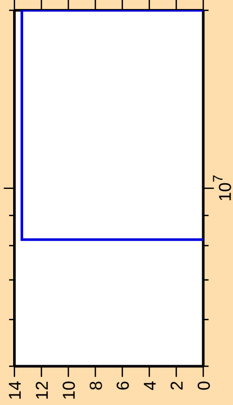
\Delta\sigma/\sigma vs. E for ^{114}\text{Sn}(n,2n)
