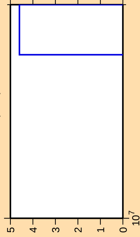
\Delta\sigma/\sigma vs. E for ^{121}\text{Sn}(n,\text{nt})
