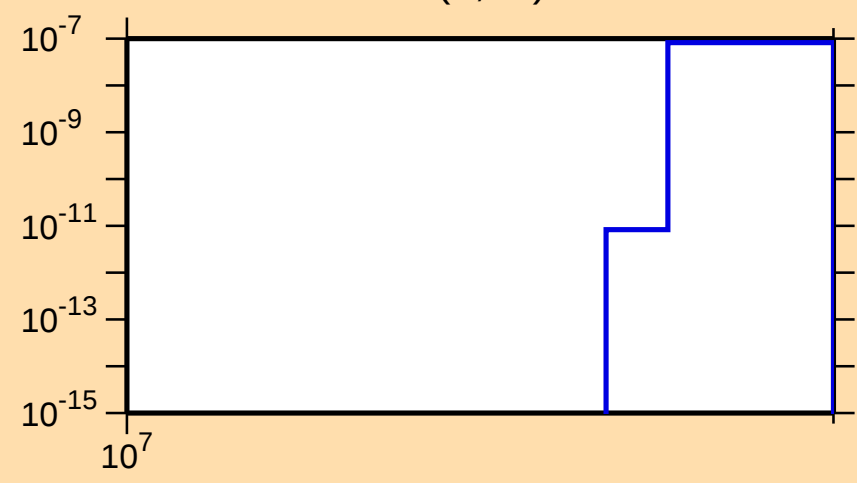
\sigma vs. E for ^{121}\text{Sn}(n,\text{nd})
