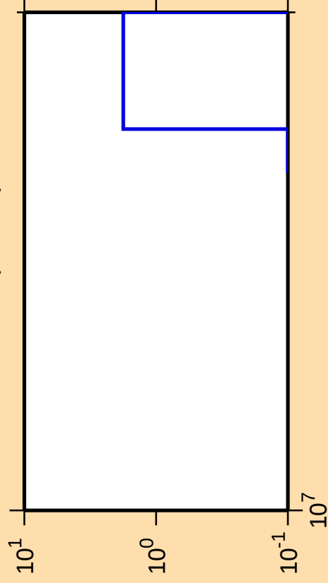
\Delta\sigma/\sigma vs. E for ^{121}\text{Sn}(n,\text{He3})
