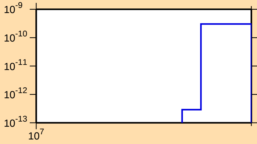
\sigma vs. E for ^{121}\text{Sn}(n,2n\alpha)
