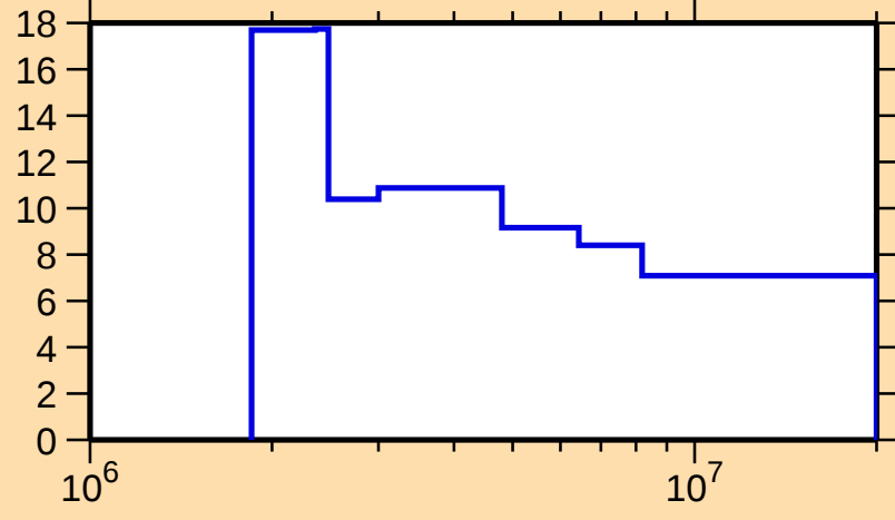
\Delta\sigma/\sigma vs. E for ^{121}\text{Sn}(n,n\text{onel.})
