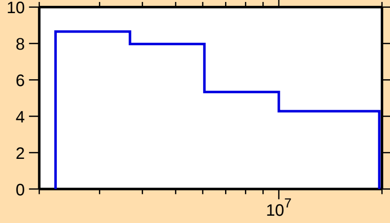
\Delta\sigma/\sigma vs. E for ^{129}\text{Sn}(n,n\text{inel.})
