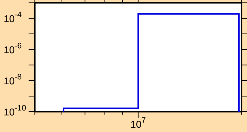
\sigma vs. E for ^{129}\text{Sn}(n,p)
