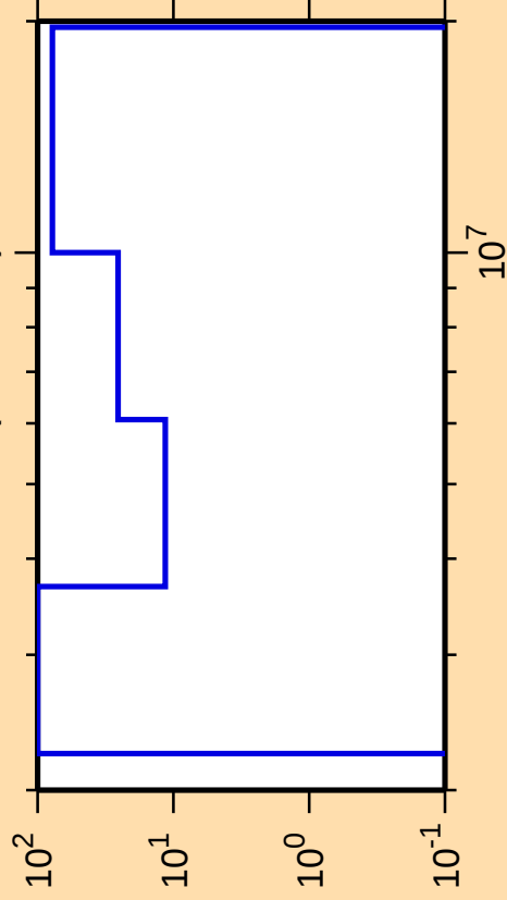
\Delta\sigma/\sigma vs. E for ^{129}\text{Sn}(n,\text{ncont.})
