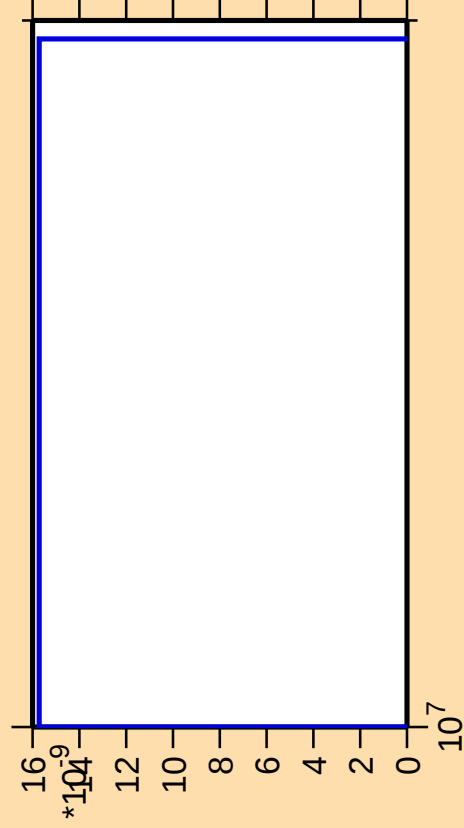
\Delta\sigma/\sigma vs. E for ^{129}\text{Sn}(n,2np)
