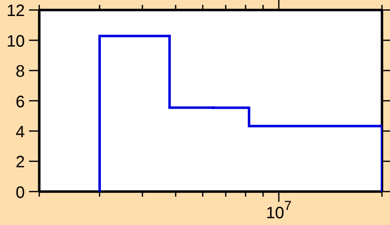
\Delta\sigma/\sigma vs. E for ^{129}\text{Sn}(n,n\text{nonel.})
