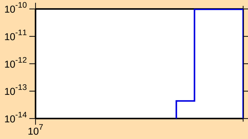
\sigma vs. E for ^{76}\text{Sr}(\text{mt } 34)
