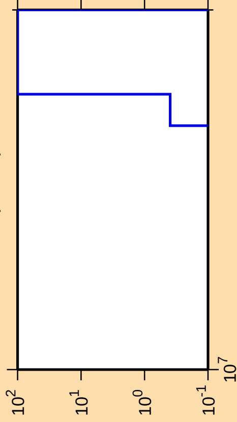
\Delta\sigma/\sigma vs. E for ^{76}\text{Sr}(\text{mt } 34)
