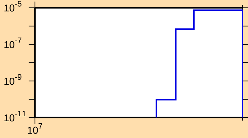
\sigma vs. E for ^{76}\text{Sr}(n,2n)
