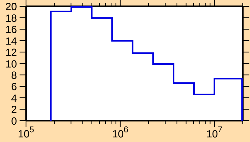
\Delta\sigma/\sigma vs. E for ^{76}\text{Sr}(\text{n,nonel.})
