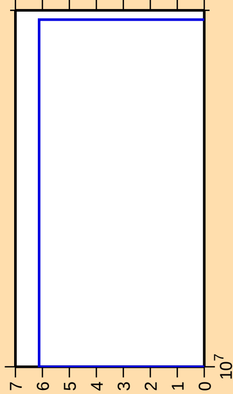
\Delta\sigma/\sigma vs. E for ^{76}\text{Sr}(\text{mt } 34)
