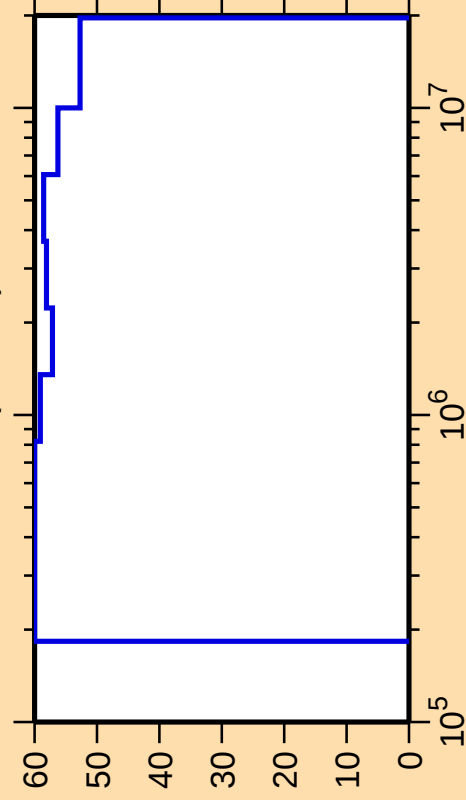
\Delta\sigma/\sigma vs. E for ^{76}\text{Sr}(\text{n,inel.})
