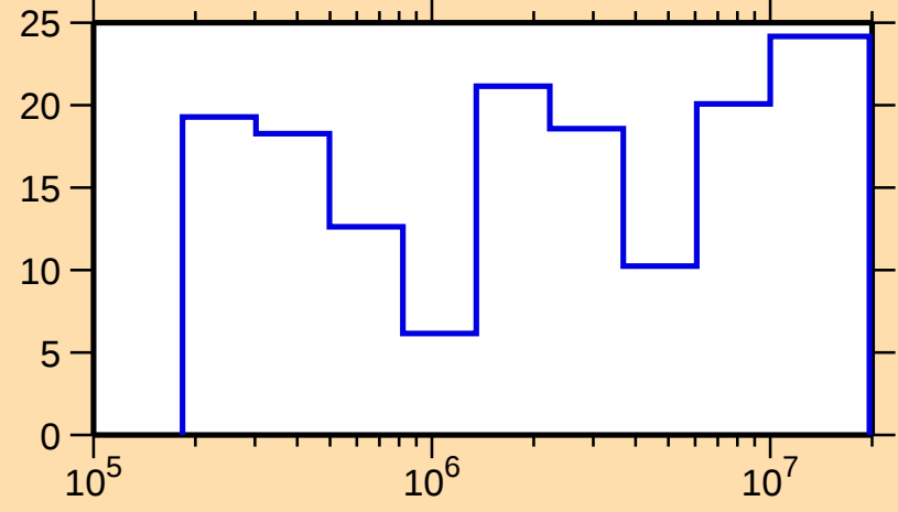
\Delta\sigma/\sigma vs. E for ^{76}\text{Sr}(\text{n,el.})
