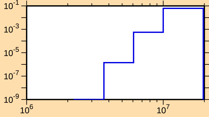
\sigma vs. E for ^{76}\text{Sr}(n,p\alpha)
