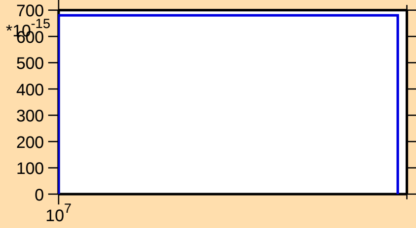
\sigma vs. E for ^{76}\text{Sr}(\text{mt } 34)
