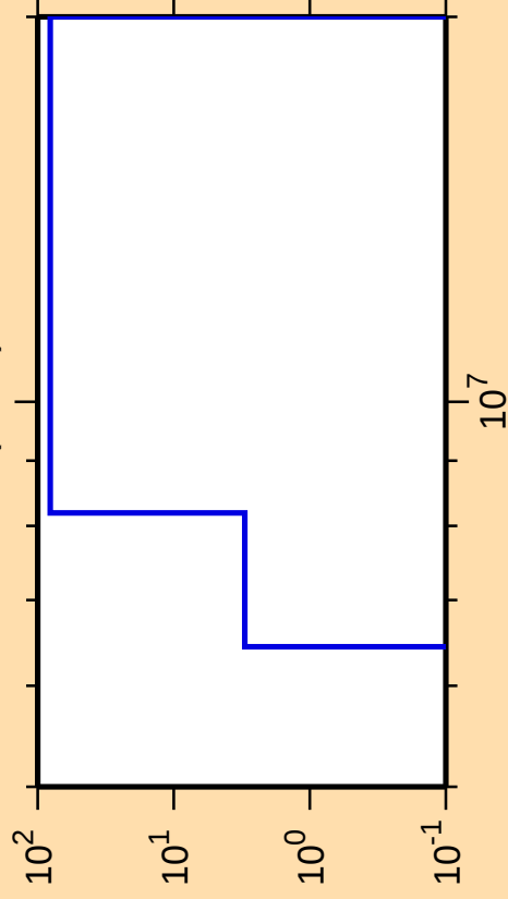
\Delta\sigma/\sigma vs. E for ^{76}\text{Sr}(n,n\alpha)
