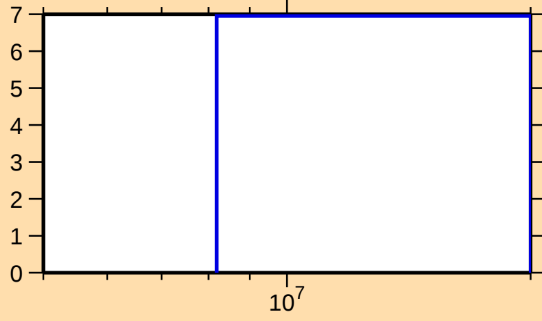
\Delta\sigma/\sigma vs. E for ^{76}\text{Sr}(n,\text{nonel.})
