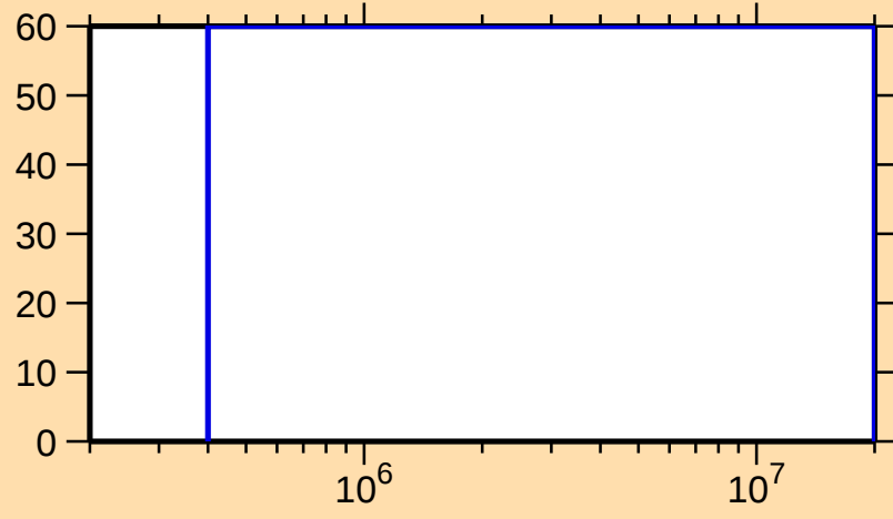
\Delta\sigma/\sigma vs. E for ^{76}\text{Sr}(n,n\text{cont.})
