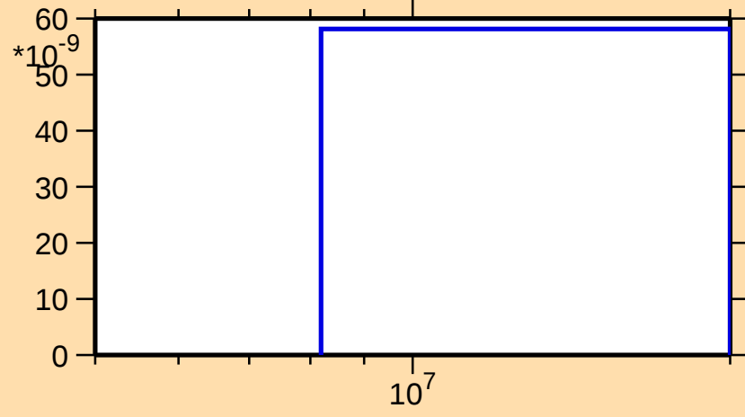
\sigma vs. E for ^{76}\text{Sr}(n,\text{pt})
