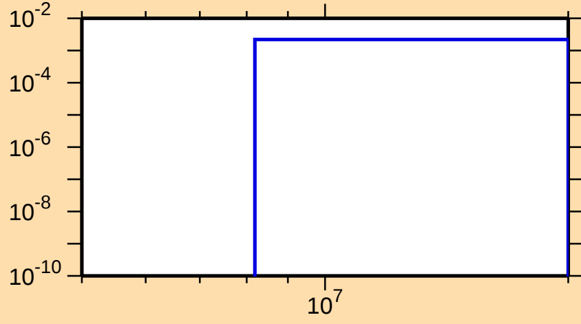
\sigma vs. E for ^{76}\text{Sr}(n,\text{pd})
