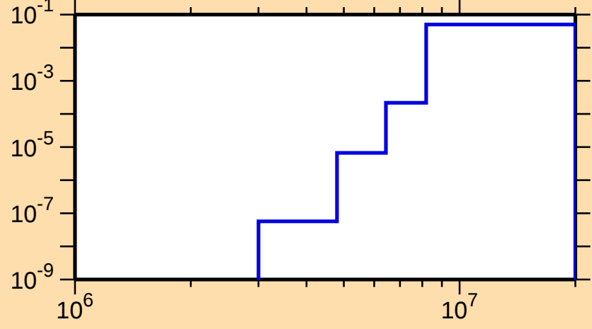
\sigma vs. E for ^{76}\text{Sr}(n,p\alpha)
