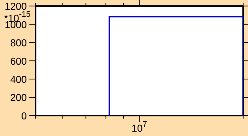
\sigma vs. E for ^{76}\text{Sr}(n,\text{nd})
