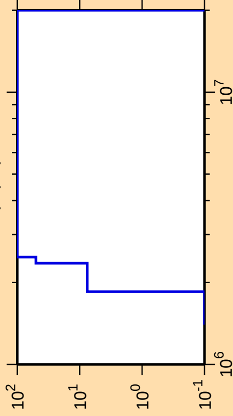
\Delta\sigma/\sigma vs. E for ^{76}\text{Sr}(n,p\alpha)
