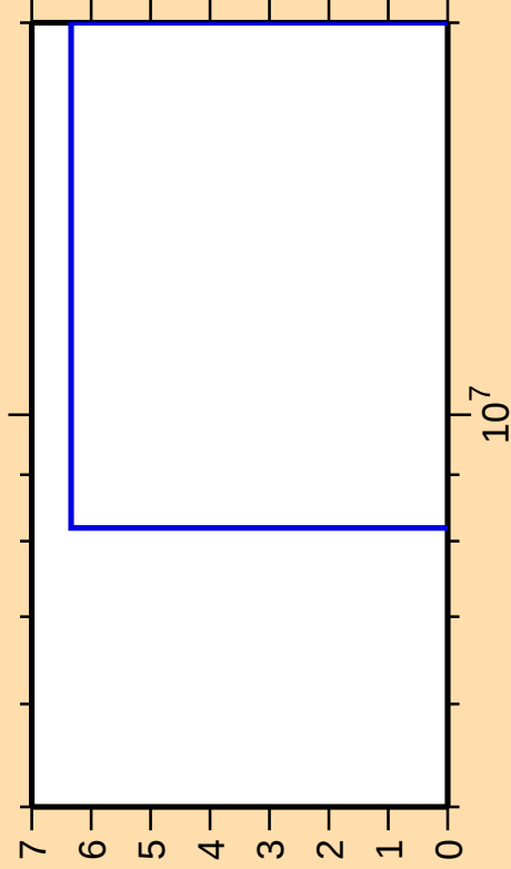
\Delta\sigma/\sigma vs. E for ^{76}\text{Sr}(n,\text{nd})
