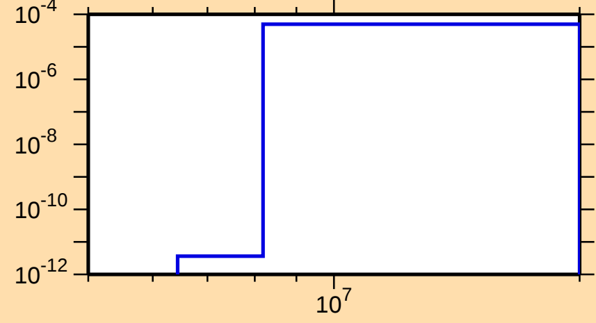
\sigma vs. E for ^{76}\text{Sr}(n,n\alpha)
