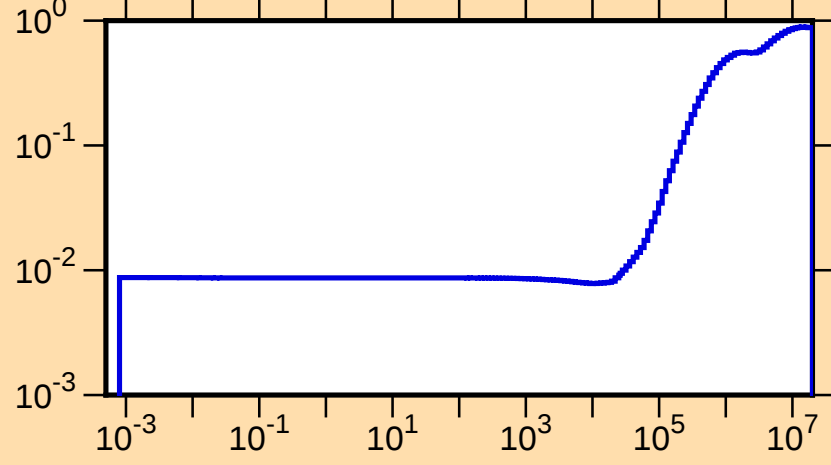
\mu vs. E for ^{77}\text{Sr}(\text{mt251})
