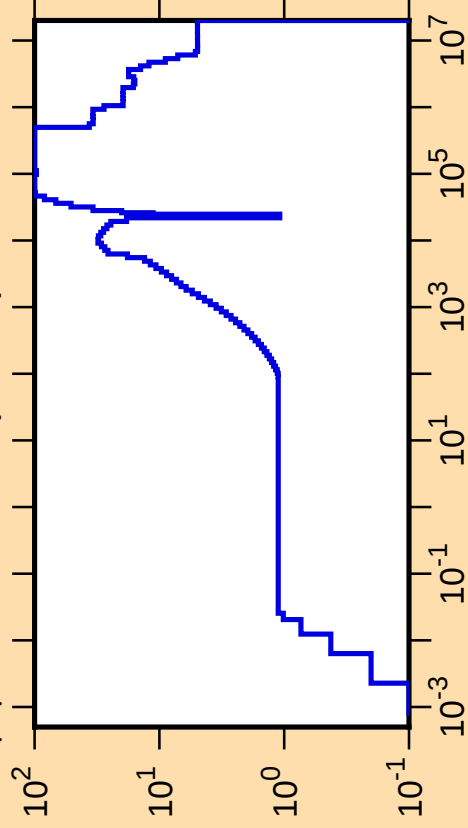
\Delta\mu/\mu vs. E for ^{77}\text{Sr}(\text{mt251})
