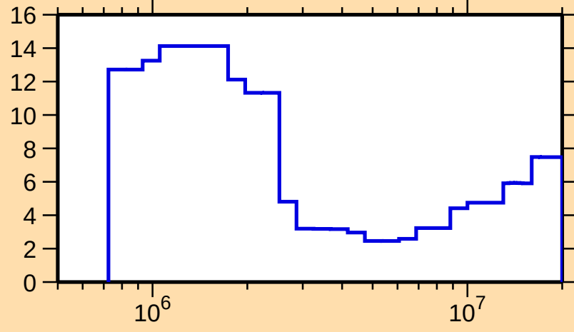
\Delta\sigma/\sigma vs. E for ^{77}\text{Sr}(n,\text{tot.})
