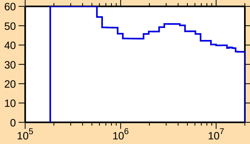
\Delta\sigma/\sigma vs. E for ^{77}\text{Sr}(n,\text{inel.})
