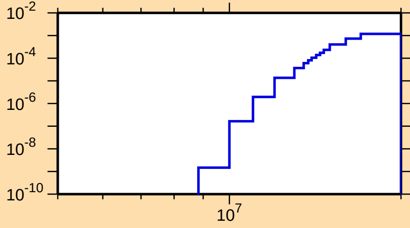
\sigma vs. E for ^{77}\text{Sr}(n,n\alpha)
