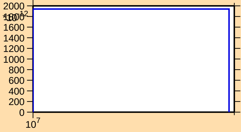
\sigma vs. E for ^{77}\text{Sr}(\text{mt } 45)
