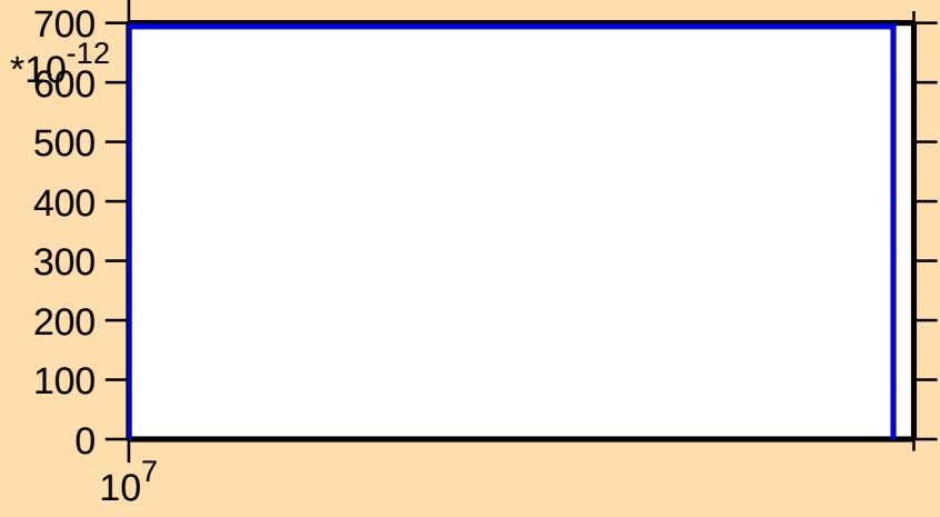
\sigma vs. E for ^{77}\text{Sr}(\text{mt } 34)
