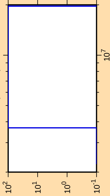
\Delta\sigma/\sigma vs. E for ^{77}\text{Sr}(n,\text{He}3)
