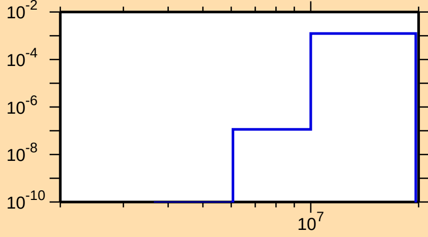
\sigma vs. E for ^{77}\text{Sr}(n,\text{He}3)
