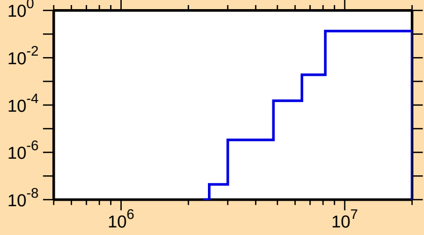
\sigma vs. E for ^{77}\text{Sr}(n,p\alpha)
