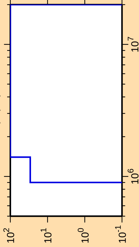
\Delta\sigma/\sigma vs. E for ^{77}\text{Sr}(n,p\alpha)
