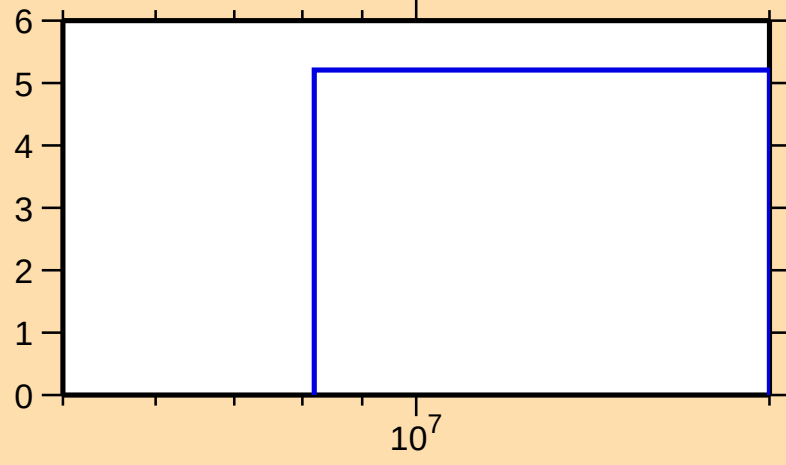
\Delta\sigma/\sigma vs. E for ^{77}\text{Sr}(n,\text{tot.})
