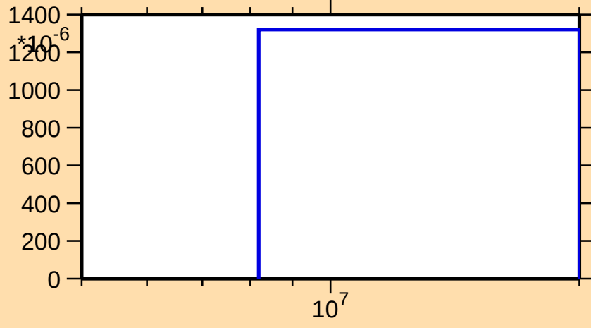
\sigma vs. E for ^{77}\text{Sr}(n,\text{pd})
