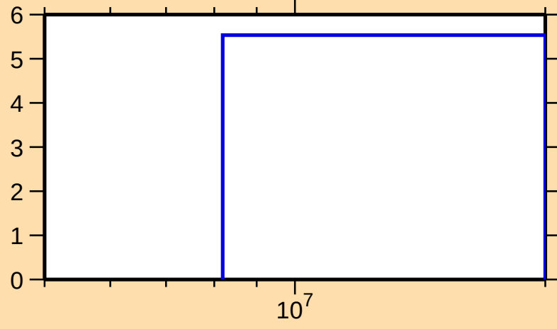
\Delta\sigma/\sigma vs. E for ^{77}\text{Sr}(n,\text{el.})
