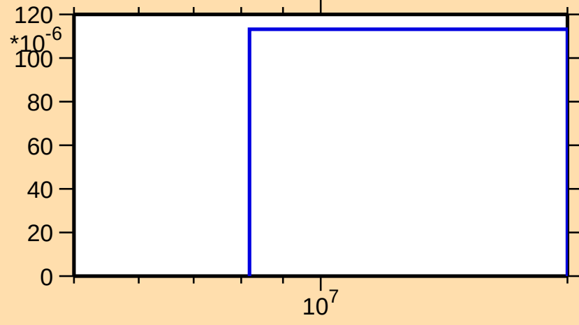
\sigma vs. E for ^{77}\text{Sr}(n,2n)
