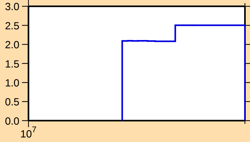
\Delta\sigma/\sigma vs. E for ^{78}\text{Sr}(n,\text{tot.})
