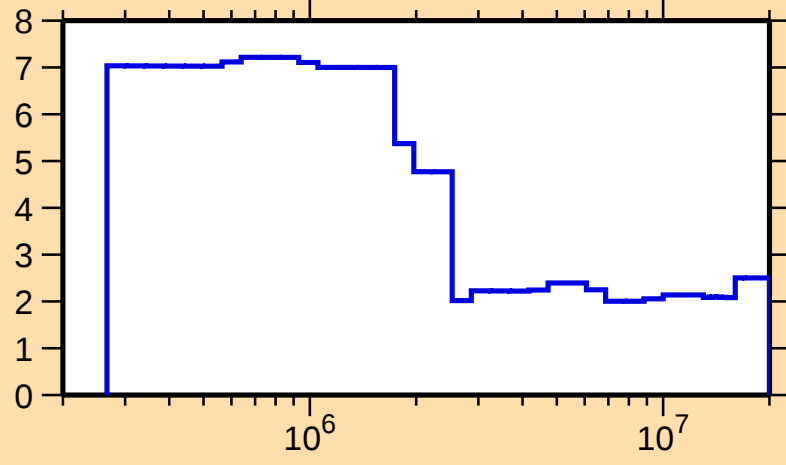
\Delta\sigma/\sigma vs. E for ^{78}\text{Sr}(n,\text{tot.})
