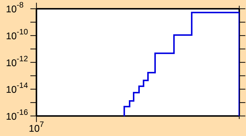
\sigma vs. E for ^{78}\text{Sr}(\text{mt117})
