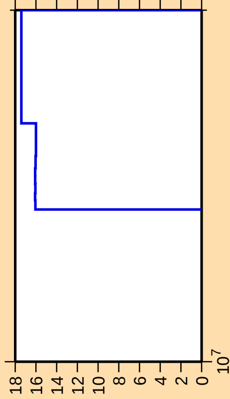
\Delta\sigma/\sigma vs. E for ^{78}\text{Sr}(n,n_1)
