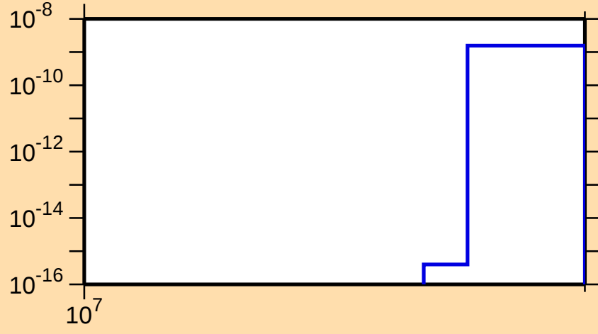
\sigma vs. E for ^{78}\text{Sr}(n,\text{nd})
