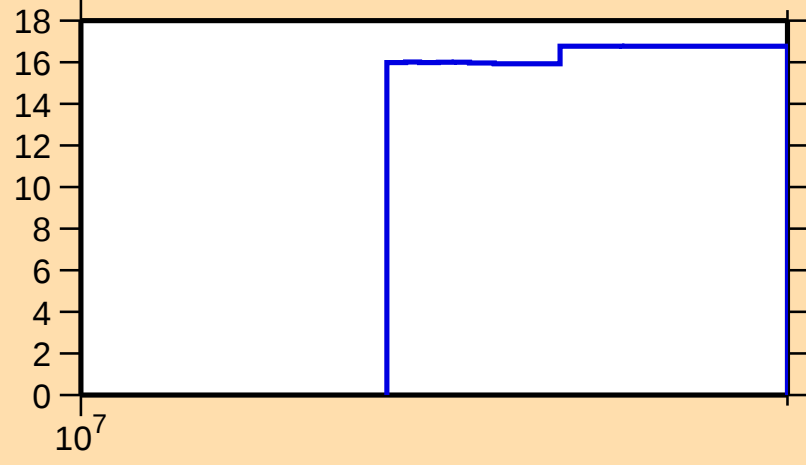
\Delta\sigma/\sigma vs. E for ^{78}\text{Sr}(n,\text{inel.})
