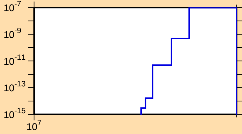
\sigma vs. E for ^{78}\text{Sr}(\text{mt } 45)
