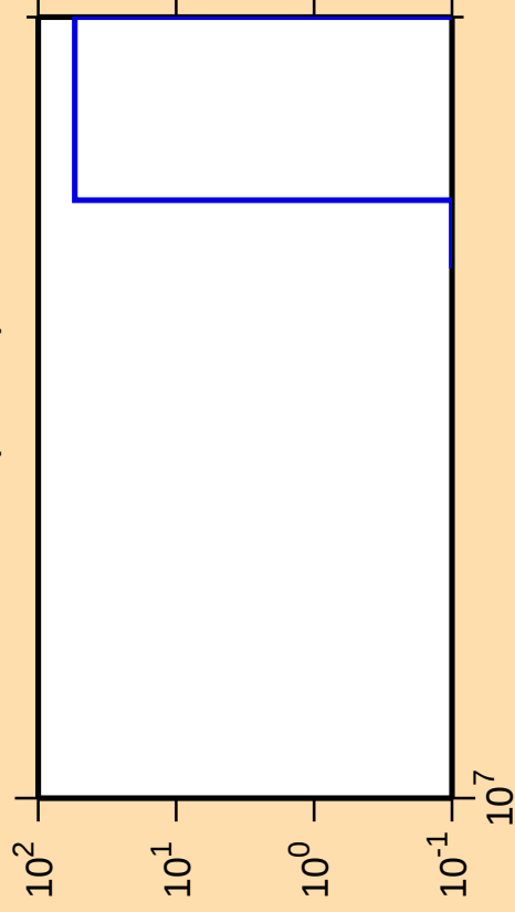
\Delta\sigma/\sigma vs. E for ^{78}\text{Sr}(\text{mt } 34)
