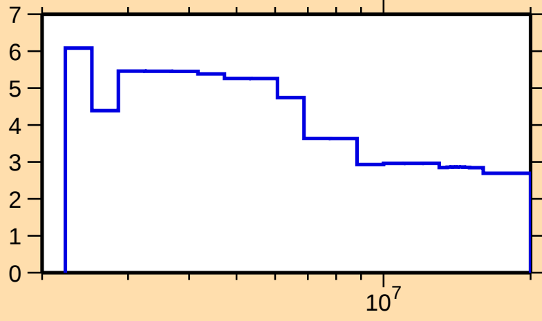
\Delta\sigma/\sigma vs. E for ^{78}\text{Sr}(n,\text{el.})
