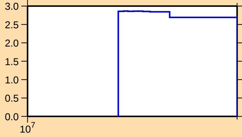
\Delta\sigma/\sigma vs. E for ^{78}\text{Sr}(n,\text{el.})
