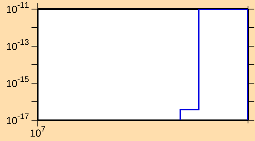
\sigma vs. E for ^{78}\text{Sr}(\text{mt } 34)
