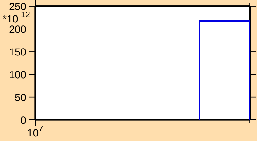
\sigma vs. E for ^{78}\text{Sr}(n,2np)
