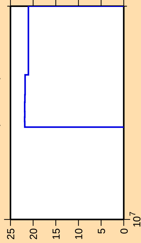
\Delta\sigma/\sigma vs. E for ^{78}\text{Sr}(n,n\text{cont.})
