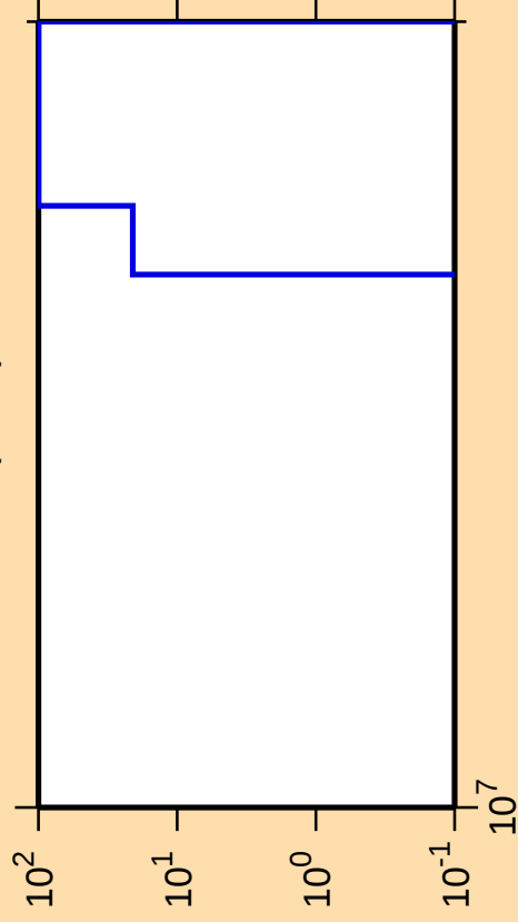
\Delta\sigma/\sigma vs. E for ^{78}\text{Sr}(n,\text{nd})
