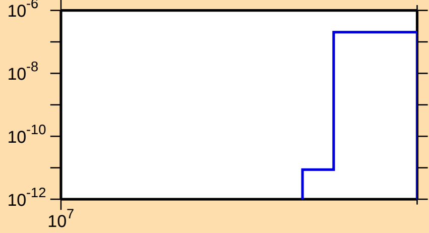
\sigma vs. E for ^{78}\text{Sr}(n,\text{pt})
