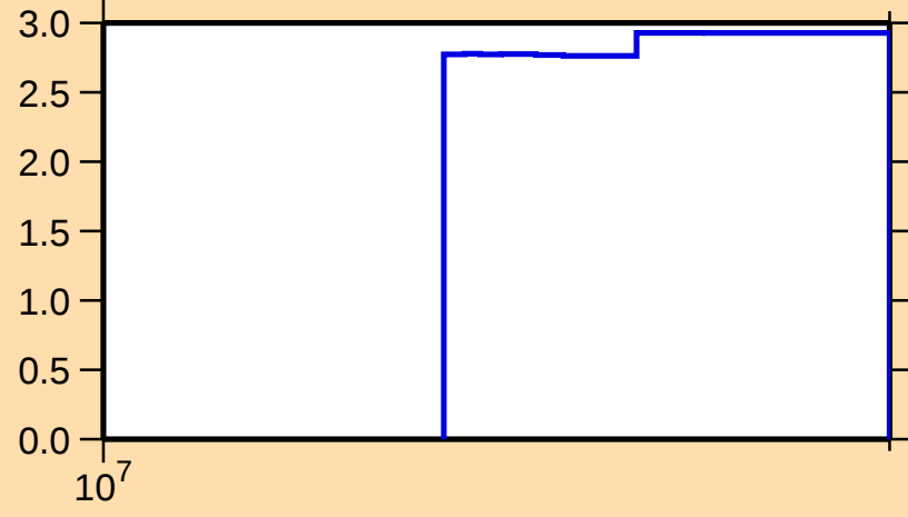
\Delta\sigma/\sigma vs. E for ^{78}\text{Sr}(n,\text{nonel.})
