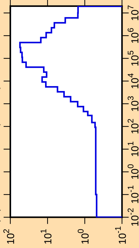
\Delta\mu/\mu vs. E for ^{78}\text{Sr}(\text{mt251})
