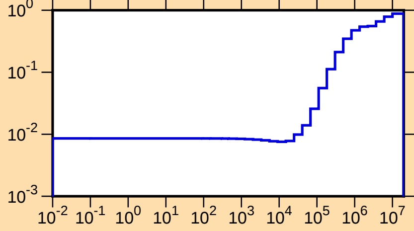
\mu vs. E for ^{78}\text{Sr}(\text{mt251})
