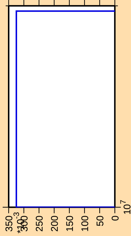
\Delta\sigma/\sigma vs. E for ^{78}\text{Sr}(\text{mt } 34)
