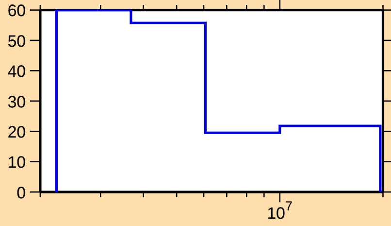
\Delta\sigma/\sigma vs. E for ^{78}\text{Sr}(n,n\text{cont.})
