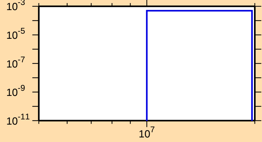
\sigma vs. E for ^{78}\text{Sr}(n,\text{pd})
