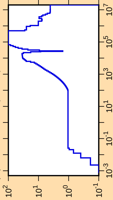
\Delta\mu/\mu vs. E for ^{79}\text{Sr}(\text{mt251})
