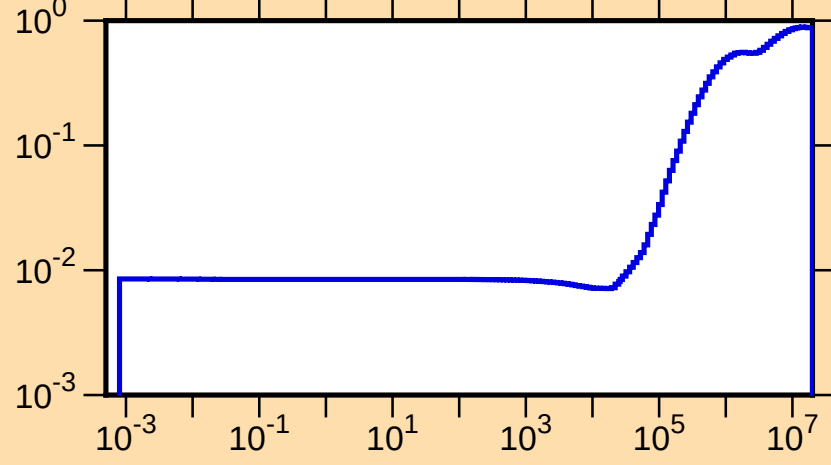
\mu vs. E for ^{79}\text{Sr}(\text{mt251})
