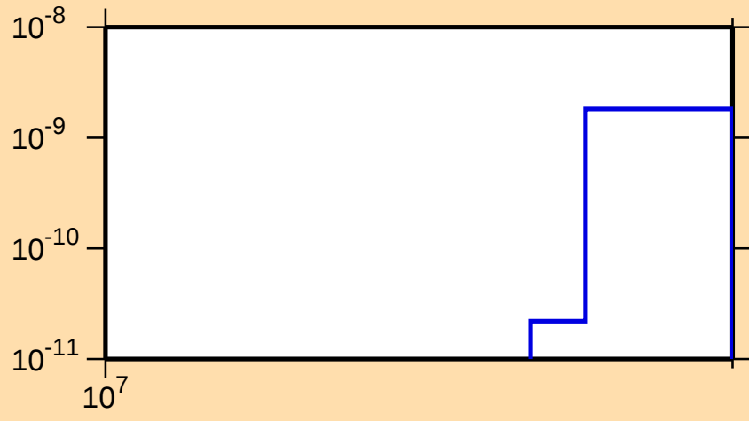
\sigma vs. E for ^{79}\text{Sr}(\text{mt117})
