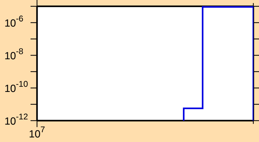
\sigma vs. E for ^{79}\text{Sr}(n,2np)
