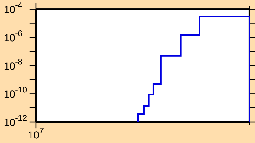
\sigma vs. E for ^{79}\text{Sr}(n,\text{pt})
