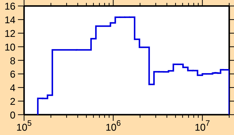
\Delta\sigma/\sigma vs. E for ^{79}\text{Sr}(\text{n,el.})
