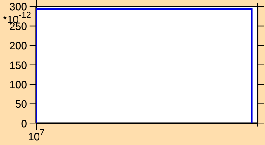
\sigma vs. E for ^{79}\text{Sr}(\text{mt } 45)
