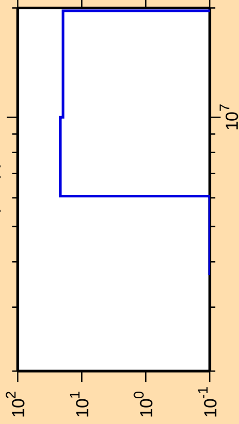
\Delta\sigma/\sigma vs. E for ^{79}\text{Sr}(n,np)
