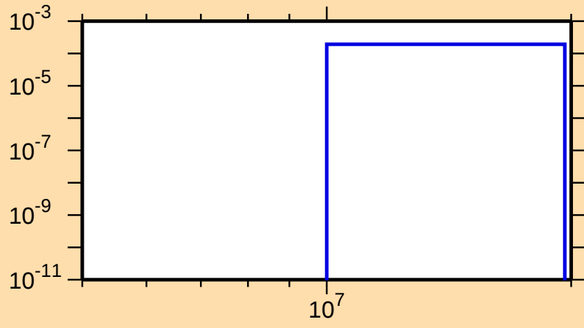
\sigma vs. E for ^{79}\text{Sr}(n,\text{pd})
