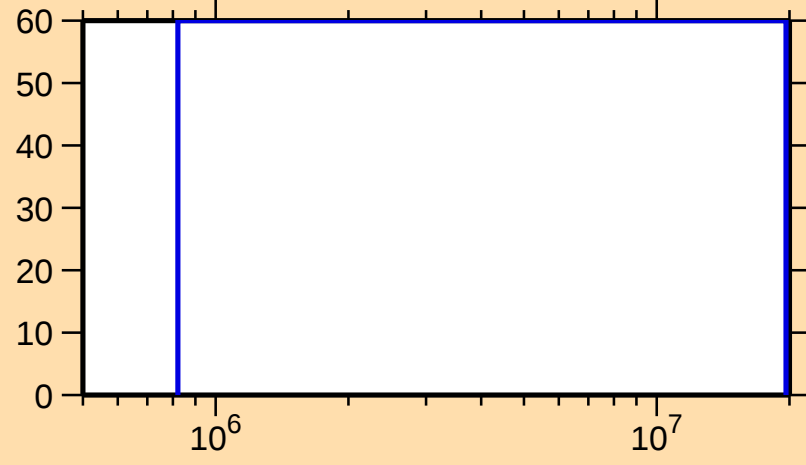
\Delta\sigma/\sigma vs. E for ^{79}\text{Sr}(n,n\text{cont.})
