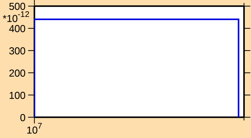
\sigma vs. E for ^{79}\text{Sr}(\text{mt } 34)
