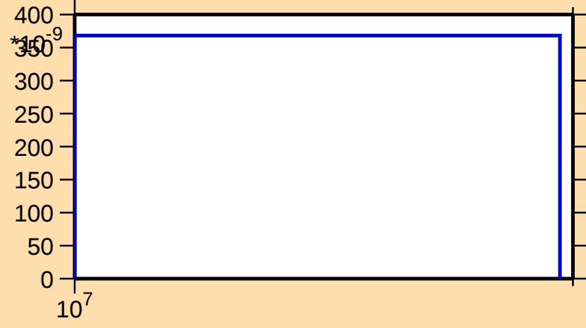
\sigma vs. E for ^{79}\text{Sr}(n,\text{pt})
