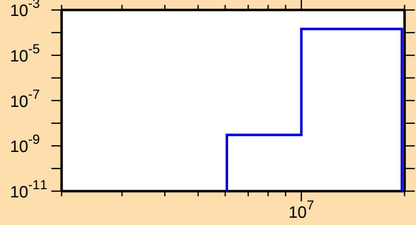
\sigma vs. E for ^{79}\text{Sr}(n,\text{He3})
