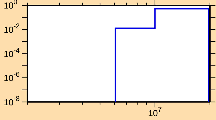
\sigma vs. E for ^{79}\text{Sr}(n,np)
