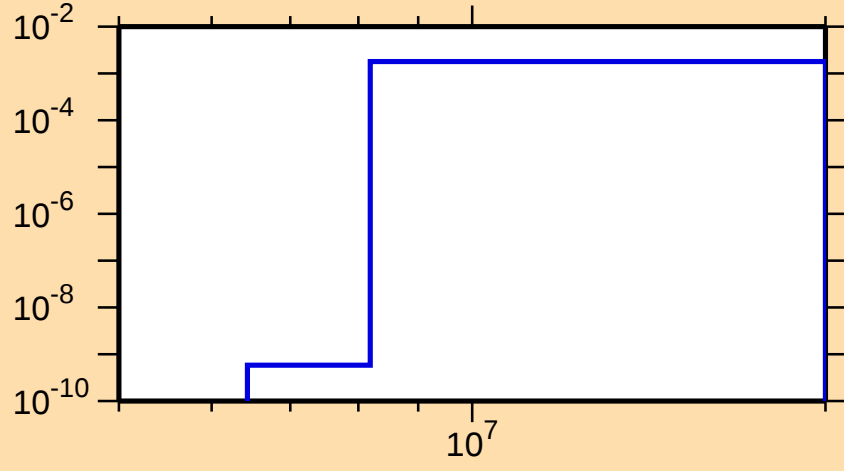
\sigma vs. E for ^{79}\text{Sr}(n,n\alpha)
