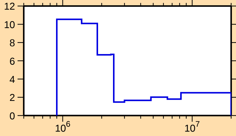
\Delta\sigma/\sigma vs. E for ^{79}\text{Sr}(n,\text{tot.})
