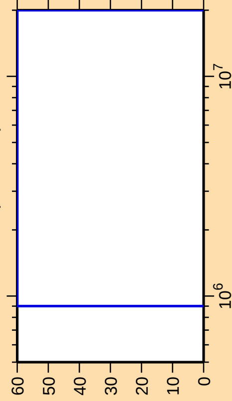
\Delta\sigma/\sigma vs. E for ^{79}\text{Sr}(n,\text{ncont.})
