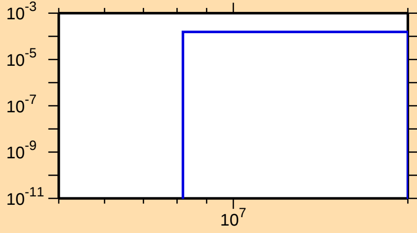
\sigma vs. E for ^{79}\text{Sr}(n,\text{pd})
