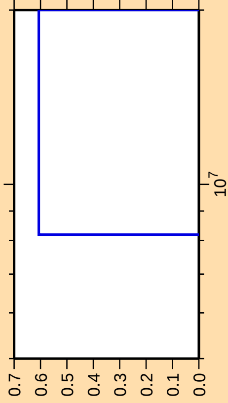
\Delta\sigma/\sigma vs. E for ^{79}\text{Sr}(n,2n\alpha)
