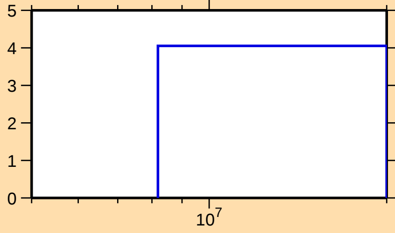
\Delta\sigma/\sigma vs. E for ^{79}\text{Sr}(n,\text{nonel.})
