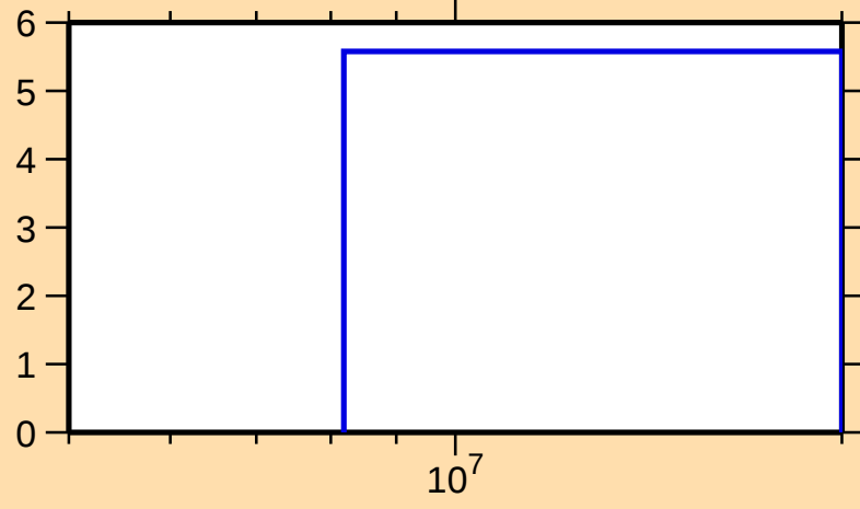
\Delta\sigma/\sigma vs. E for ^{79}\text{Sr}(n,\text{el.})
