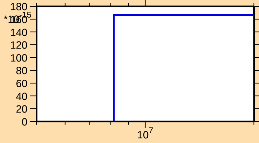
\sigma vs. E for ^{79}\text{Sr}(n,2n\alpha)
