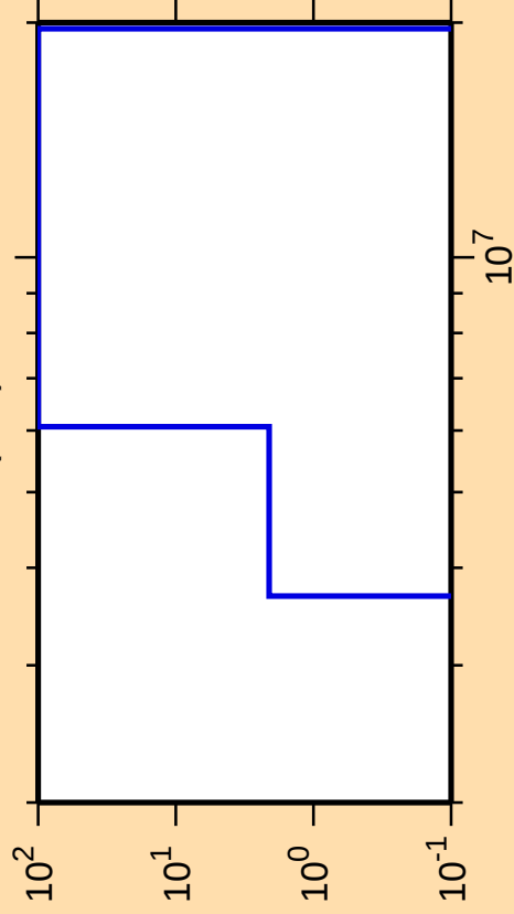
\Delta\sigma/\sigma vs. E for ^{80}\text{Sr}(n,d)
