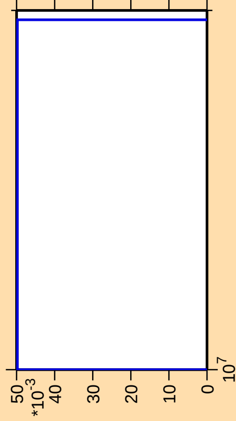
\Delta\sigma/\sigma vs. E for ^{80}\text{Sr}(n,2np)
