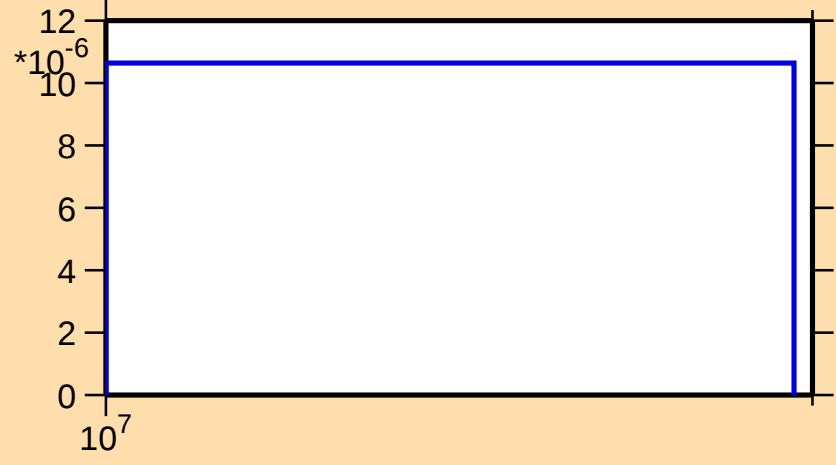
\sigma vs. E for ^{80}\text{Sr}(n,t)
