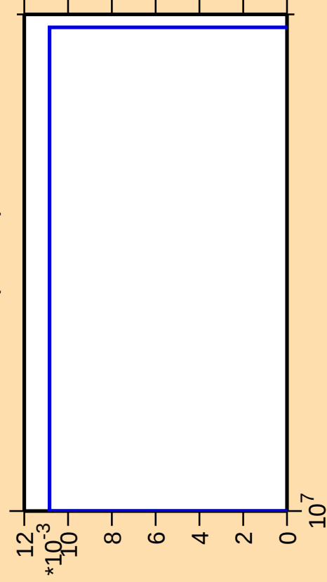
\Delta\sigma/\sigma vs. E for ^{80}\text{Sr}(\text{mt } 34)
