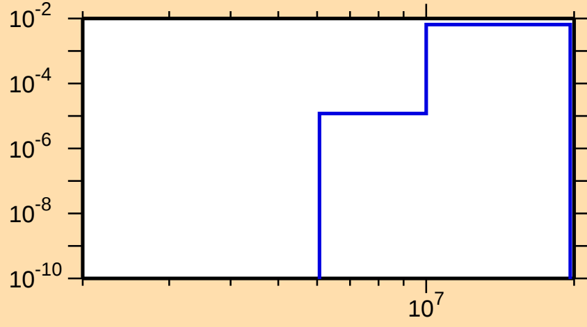
\sigma vs. E for ^{80}\text{Sr}(n,d)
