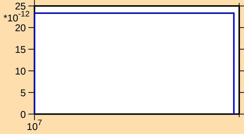
\sigma vs. E for ^{80}\text{Sr}(\text{mt } 45)
