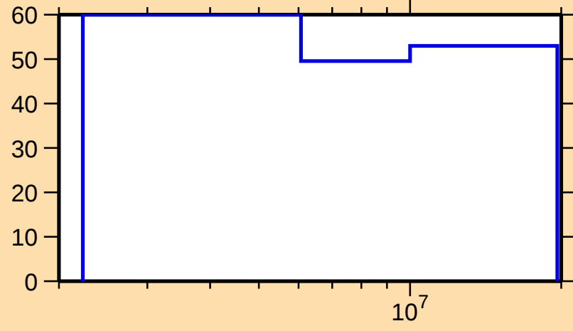
\Delta\sigma/\sigma vs. E for ^{80}\text{Sr}(n,n\text{cont.})
