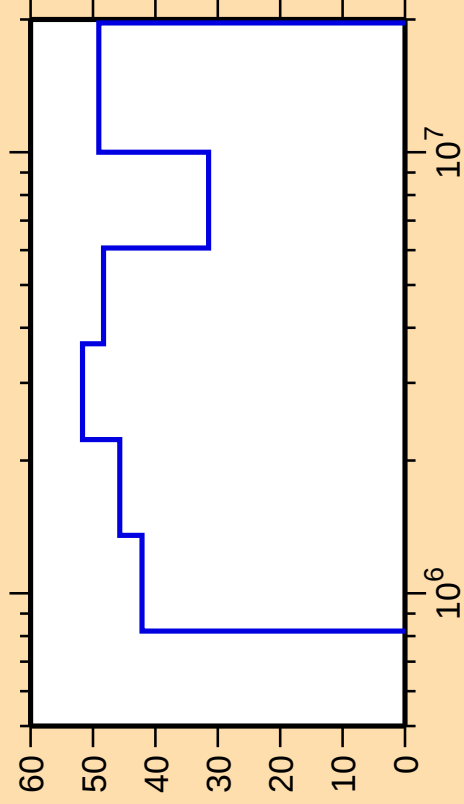
\Delta\sigma/\sigma vs. E for ^{80}\text{Sr}(n,n_4)
