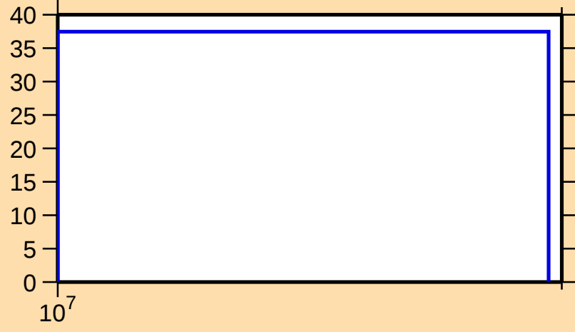
\Delta\sigma/\sigma vs. E for ^{80}\text{Sr}(n,\text{inel.})
