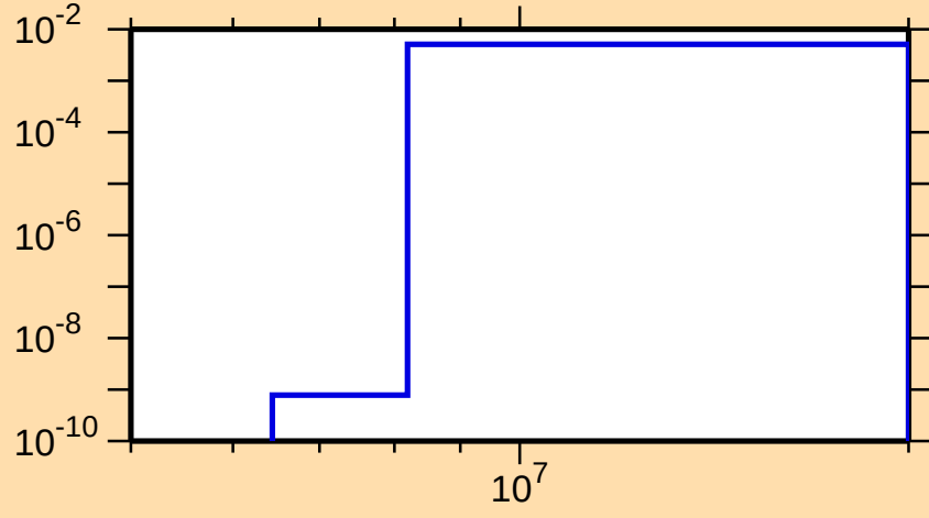
\sigma vs. E for ^{80}\text{Sr}(n,n\alpha)
