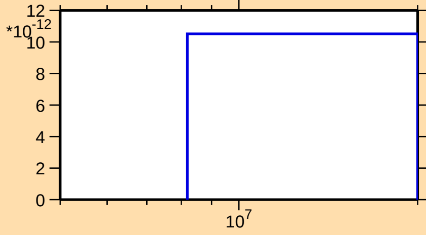
\sigma vs. E for ^{80}\text{Sr}(n,\text{pt})
