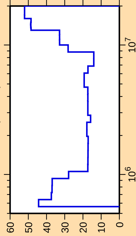
\Delta\sigma/\sigma vs. E for ^{82}\text{Sr}(\text{n,inel.})
