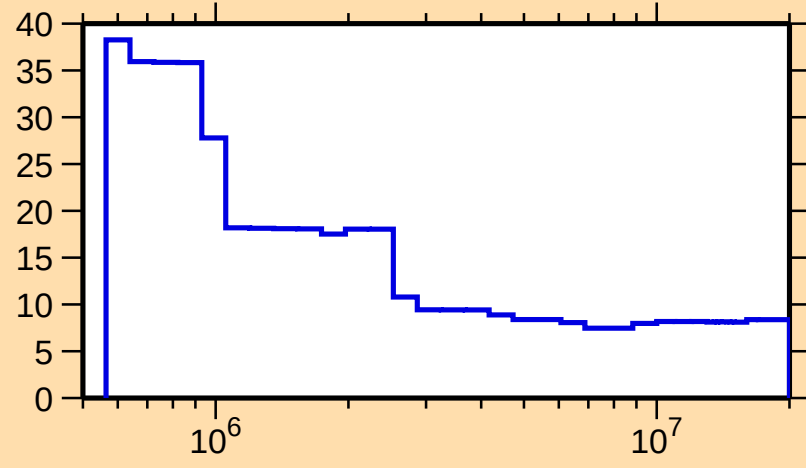
\Delta\sigma/\sigma vs. E for ^{82}\text{Sr}(\text{n,nonel.})
