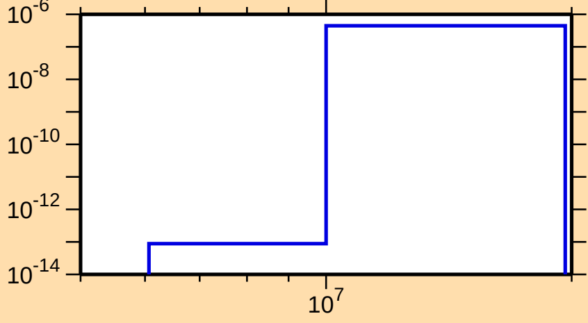
\sigma vs. E for ^{82}\text{Sr}(n,\text{He}3)
