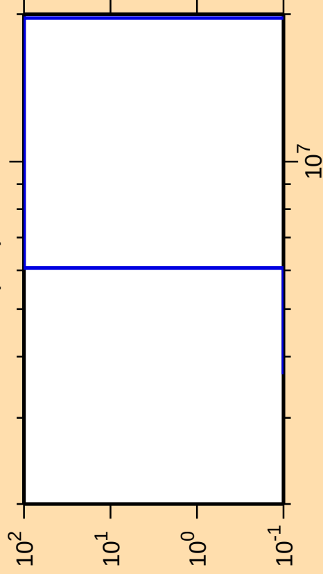
\Delta\sigma/\sigma vs. E for ^{82}\text{Sr}(n,d)
