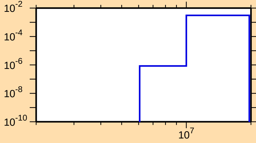
\sigma vs. E for ^{82}\text{Sr}(n,d)
