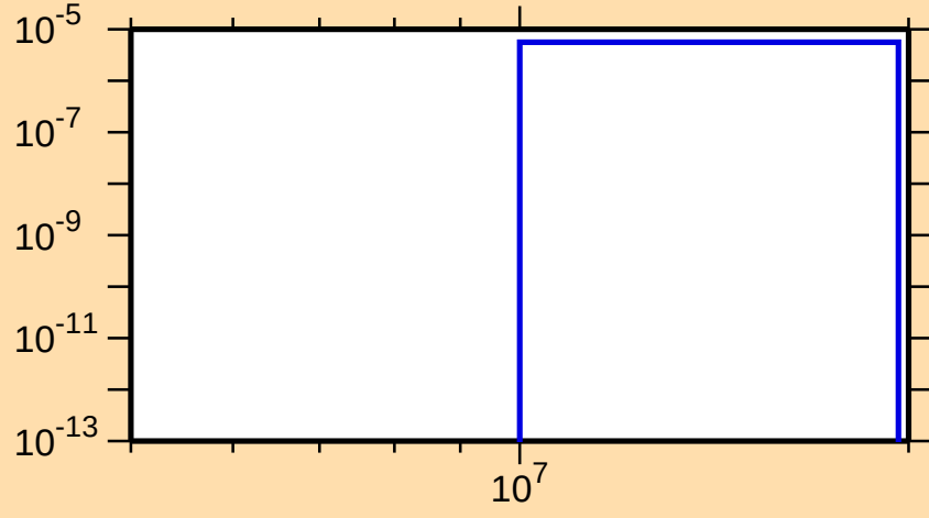
\sigma vs. E for ^{82}\text{Sr}(n,p\alpha)
