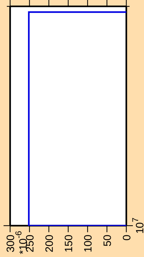
\Delta\sigma/\sigma vs. E for ^{82}\text{Sr}(n,2np)
