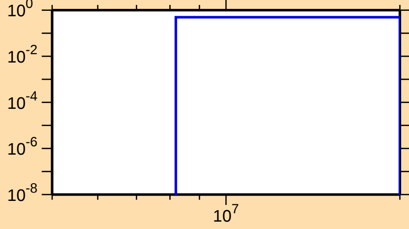
\sigma vs. E for ^{82}\text{Sr}(n,np)
