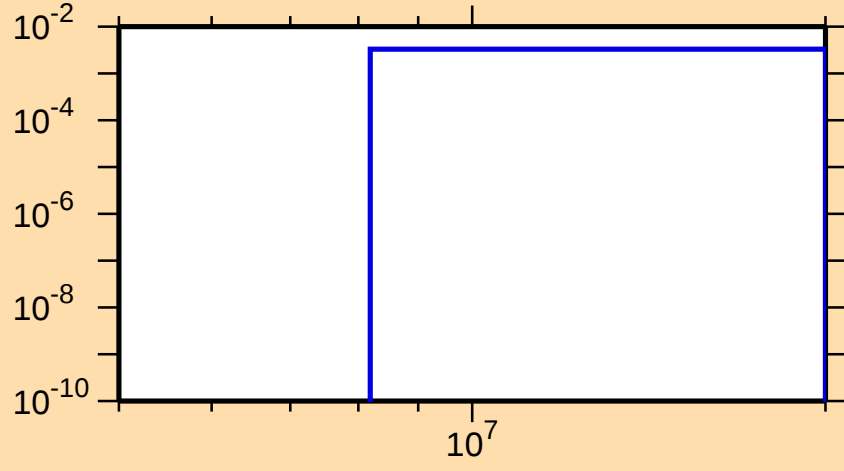
\sigma vs. E for ^{82}\text{Sr}(n,n\alpha)
