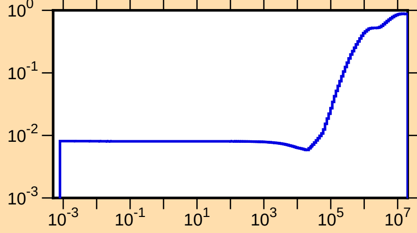
\mu vs. E for ^{83}\text{Sr}(\text{mt251})
