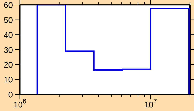
\Delta\sigma/\sigma vs. E for ^{83}\text{Sr}(n,n\text{cont.})
