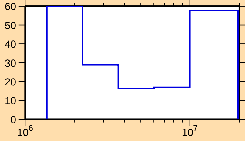
\Delta\sigma/\sigma vs. E for ^{83}\text{Sr}(n,ncont.)
