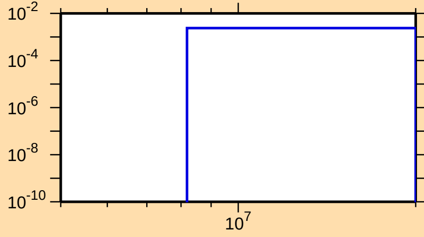
\sigma vs. E for ^{83}\text{Sr}(n,n\alpha)
