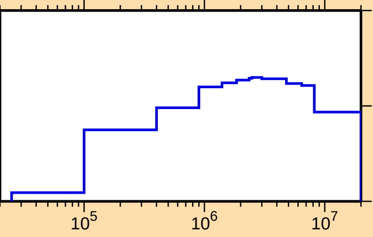
\sigma vs. E for ^{83}\text{Sr}(n,\text{inel.})
